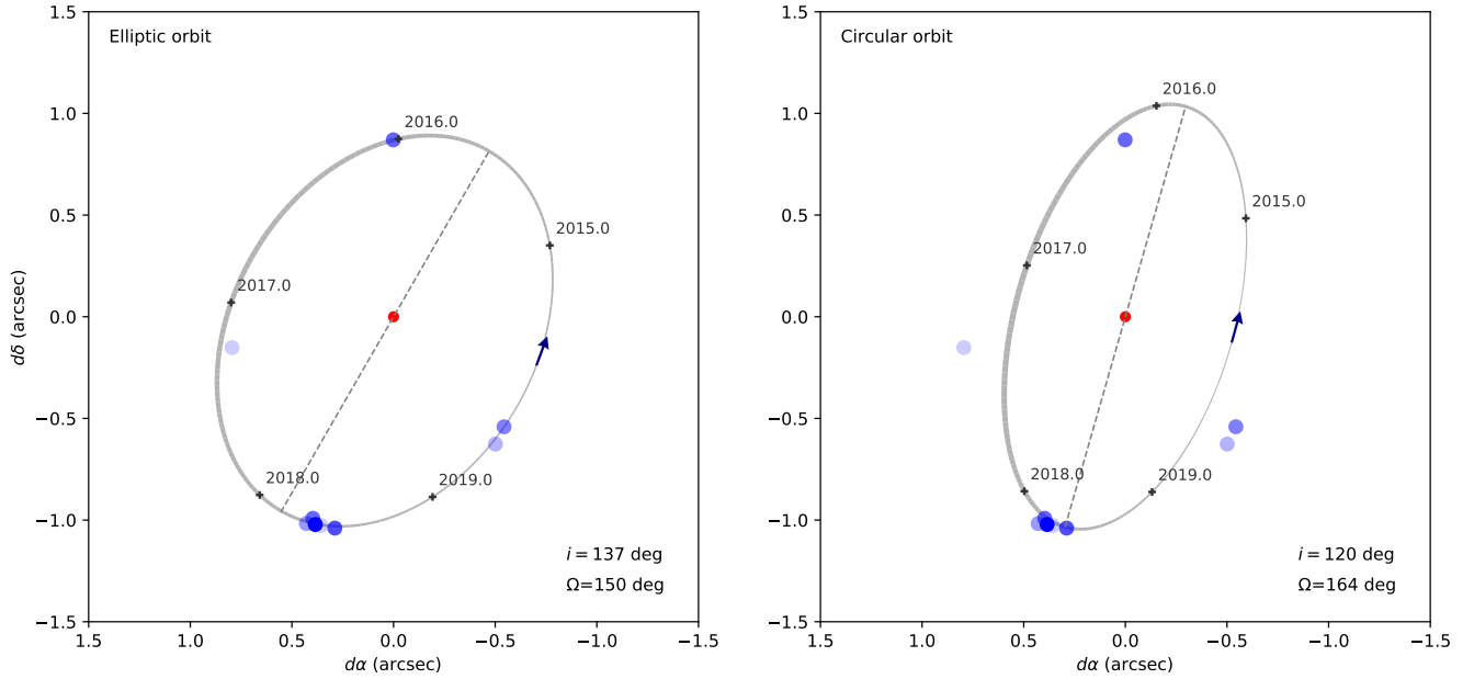
Fig. 5. Comparison between the proposed orbits for the candidate counterpart of Proxima c and the observations listed in Table 2. The density of the blue color of the points is proportional to the S/N in the individual epochs. Left panel: eccentric orbit. Right panel: circular orbit.
