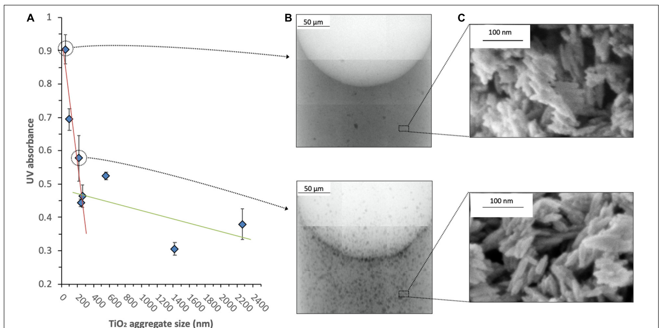
FIGURE 3 | Effect of TiO 2 nanoparticle aggregate size on the UV absorption efficacy. Different commercial nanoparticulate TiO 2 UV-filters were dispersed in a sunscreen oil phase. The UV absorption at the wavelength of 270 nm was measured by UV/vis spectrophotometer; it is plotted according to the aggregate size measured by dynamic light scattering ( A ). The resulting homogeneity of the w/o sunscreen formulation was analyzed at the micrometric aggregate scale by 2D X-ray nano-tomography ( B ). The top pictures show a finely dispersed UV-filter leading to homogeneous sunscreen and maximum UV absorption, while the bottom pictures correspond to an aggregated UV-filter leading to a heterogeneous sunscreen and lowered UV absorption (Catalano, 2020). However, both top and bottom UV-filters display similar primary nanoparticle structure at the nm scale, as observed by HR-scanning electron microscopy ( C ).
