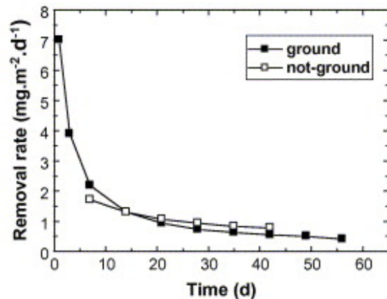
Fig. 6. Dynamic leaching test results on sintered samples.
