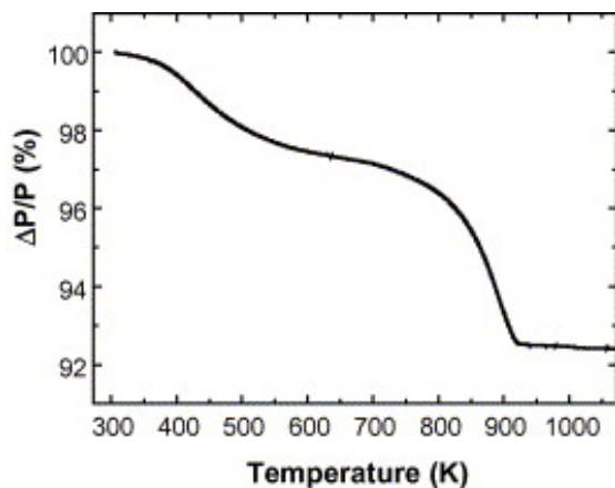
Fig. 1. TG-DTA traces of a 20 wt% sample.
