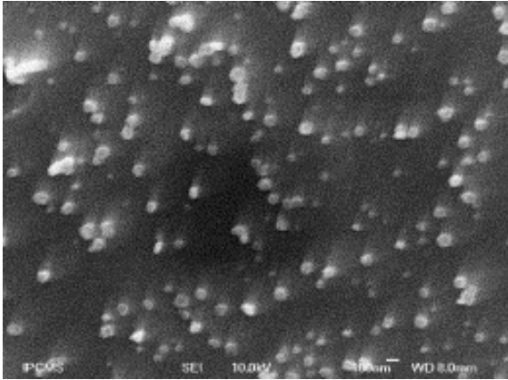
Fig. 4. SEM observation on leached sintered sample after 64 days.
