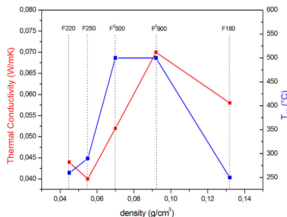
Fig. 6. Thermal conductivity and T_{10} values (derived from TGA at 10 ^\circ C min^{-1} between 25 and 1000 °C under 50 mL min^{-1} air flow) as a function of the bulk density ( \rho ) of 5 samples of humins foam.
