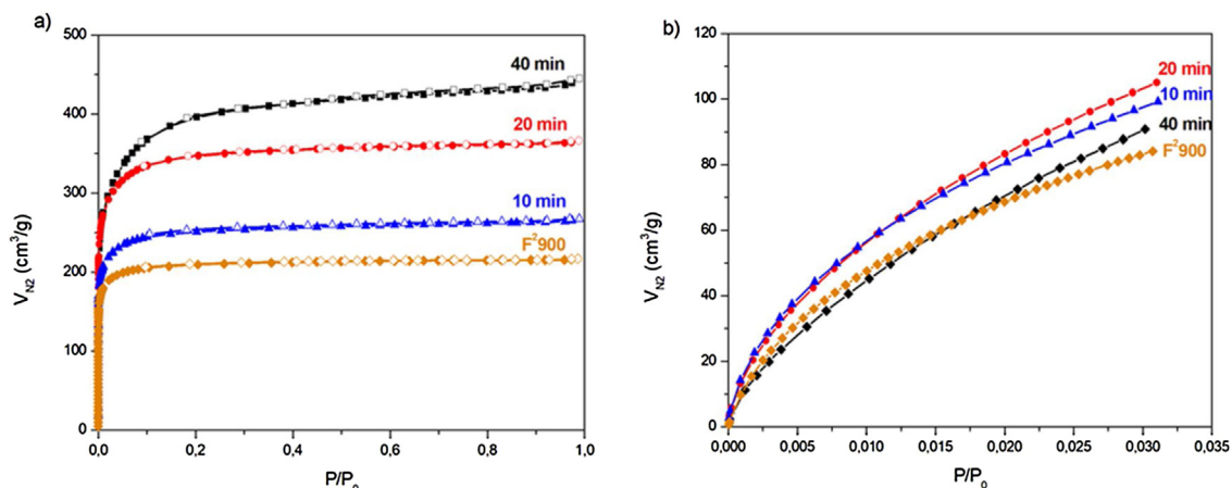
Fig. 9. N 2 adsorption of F 2 900 and derived activated carbon monoliths produced after 20 and 40 min of CO 2 treatment at 900 °C.
