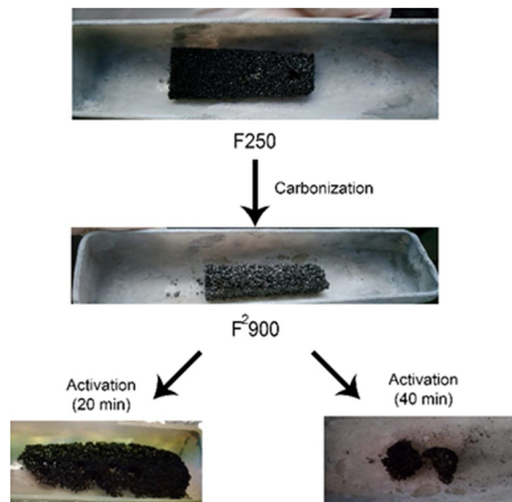
Fig. 8. Activated carbon monoliths produced with 20 and 40 min of CO 2 treatment at 900 °C.
