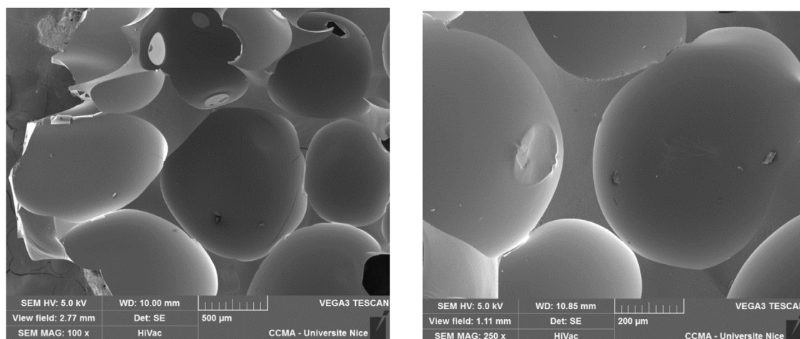
Fig. 1. SEM images of F250 humins foam.
