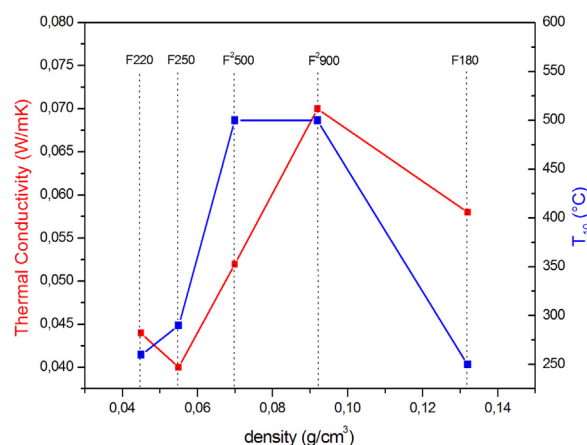
Fig. 6. Thermal conductivity and T_{10} values (derived from TGA at 10 °C min^{-1} between 25 and 1000 °C under 50 mL min^{-1} air flow) as a function of the bulk density ( \rho ) of 5 samples of humins foam.
