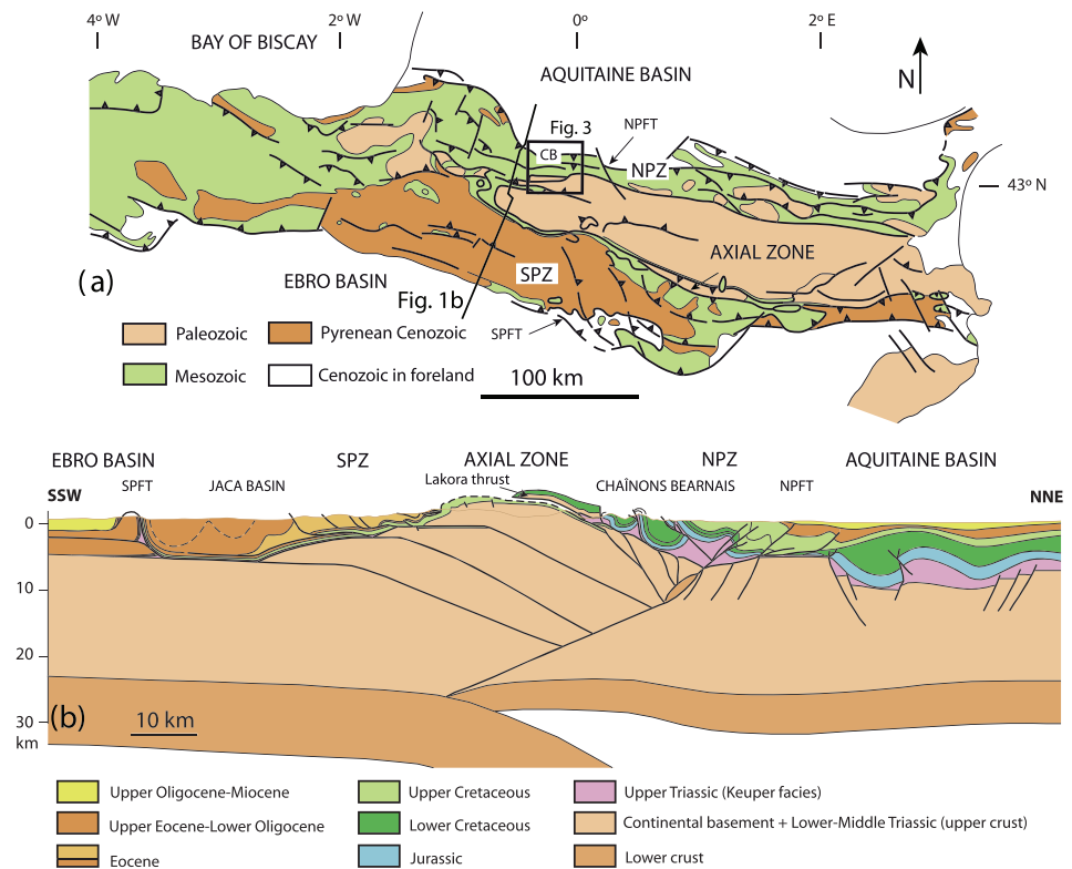
Figure 1. a) Geological map of the Pyrenees (modified from Teixell, 1998) with location of the study area (black rectangle). CB, Chainons Béarnais; NPFT, North Pyrenean frontal thrust; NPZ, North Pyrenean Zone; SPFT, South Pyrenean frontal thrust; SPZ, South Pyrenean Zone. (b) Crustal-scale cross-section across the western Axial Zone (from Teixell et al., 2016). See location in Figure 1a.
