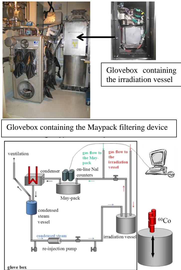
Figure 3: Scheme of the EPICUR facility.
