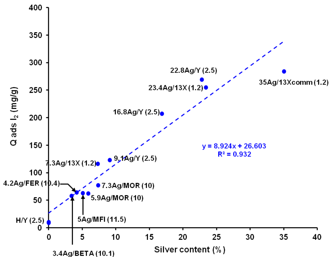
Figure 7: I 2 adsorption capacities ( [I_2]_0 = 400 ppm, m = 75 mg, V = 50 mL, T = 25^\circ\text{C} , t_{\text{eq}} = 24 h) in function of silver content for the exchanged-silver zeolites.
