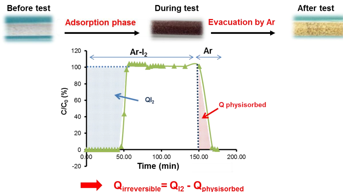
Figure 2: Typical breakthrough and desorption profiles observed during gas-phase I_2 sorption experiments and associated color changes in zeolite bed.
