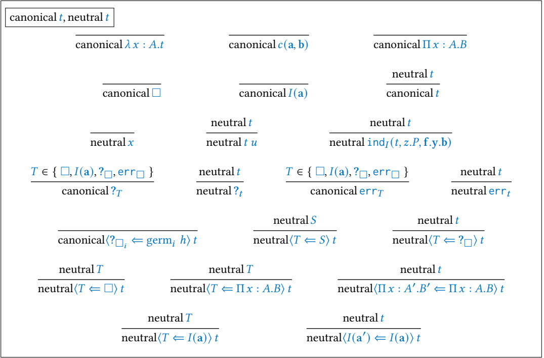
Fig. 7. Head neutral and canonical forms for CastCIC
