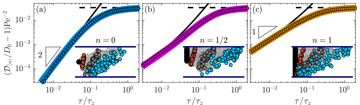
Figure 6: Reduced dispersion coefficients. as a function of dimensionless time obtained from the Langevin simulations, Eqs. (23) and (24) studied for fractions (a) n = 0 , (b) n = 1/2 , and (c) n = 1 of the channel height. The black dashed and solid lines respectively correspond to the asymptotic behaviors for the long- and short-time regimes predicted by Eqs. (4) and (10). The solid colored lines show the dispersion coefficients predicted by Eq. (15) from the moment theory for the corresponding initial conditions. The insets schematically show three instants of particle trajectories advected from the associated observation zone in a linear shear flow and with diffusion in z . The slope triangles in (a) and (c) respectively denote power-law exponents 2 and 1.
