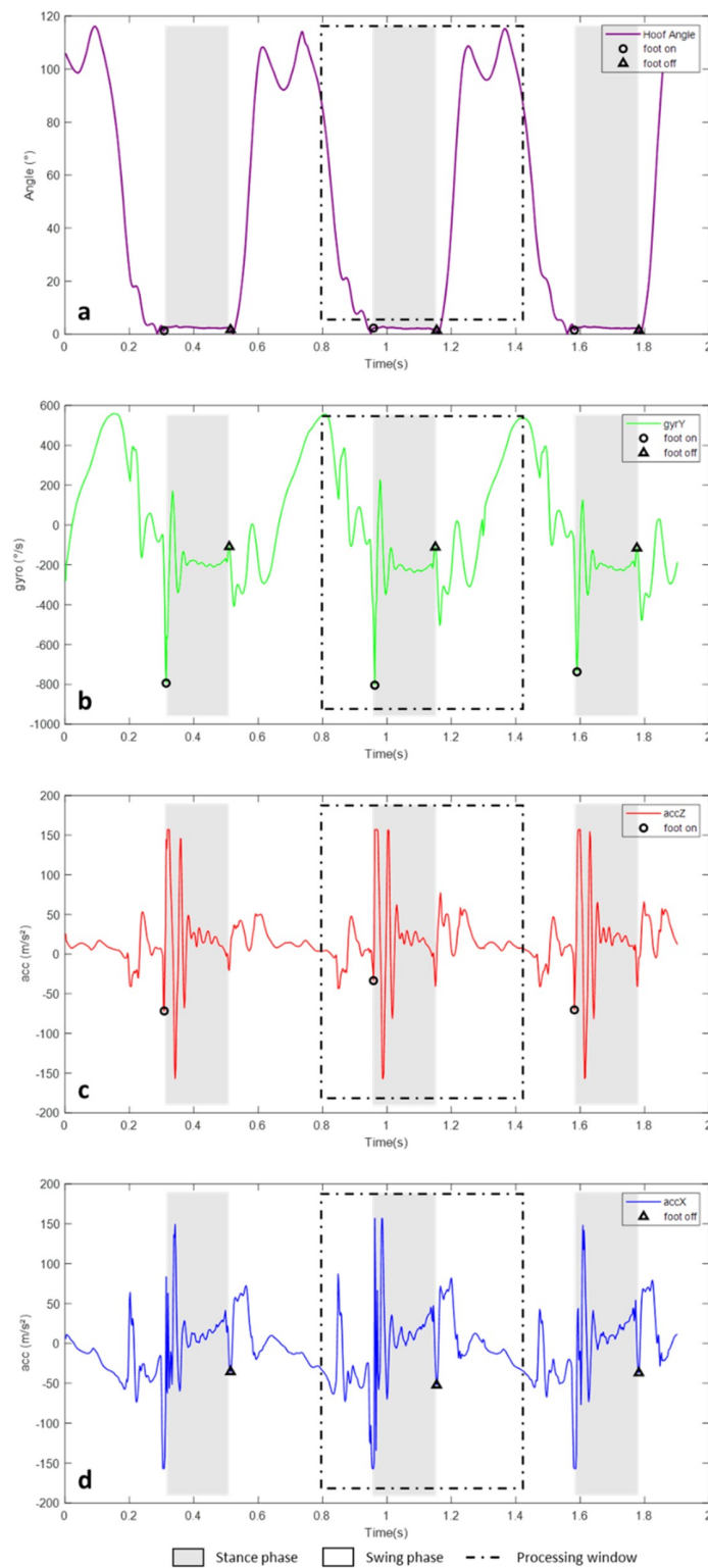
Figure 4. Representation of (a) the hoof angle calculated from the hoof markers allowing the detection of Foot on (o) and Foot off ( \Delta ) reference events ( MoCapFootOn and MoCapFootOff ), (b) the Y-axis gyrosopic signal used for the detection of Foot on (o) and Foot off ( \Delta ) events in method A ( ImuFootOn_A and ImuFootOff_A ) and method C ( ImuFootOn_C and ImuFootOff_C ), (c) the Z-axis accelerometric signal used for detection of Foot on (o) events in method B ( ImuFootOn_B ) and method D ( ImuFootOn_D ), (d) the X-axis accelerometric signal used for detection of Foot off ( \Delta ) events in method B ( ImuFootOff_B ) and method D ( ImuFootOff_D ).
