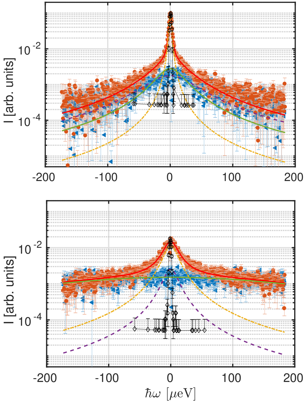
Figure 1: First spectrum (circle symbols) from a BSA protein solution in D_2O recorded using the new BATS option of IN16B in a single tube of the position-sensitive detector (PSD); top: PSD tube number 1, q = 0.44 \text{ \AA}^{-1} ; bottom: PSD tube 14, q = 1.79 \text{ \AA}^{-1} . The square symbols denote the corresponding pure D_2O solvent reference spectrum. The red solid line superimposed on the BSA/ D_2O spectrum denotes the fit of equation 1 consisting of the Lorentzian contributions with the widths \gamma , \Gamma , and \gamma_{D_2O} , respectively, assigned to the global diffusion (dashed line), internal diffusion (dash-dotted line) and water contribution (solid line superimposed on the D_2O spectrum). The diamond symbols represent the resolution function measured using Vanadium.
