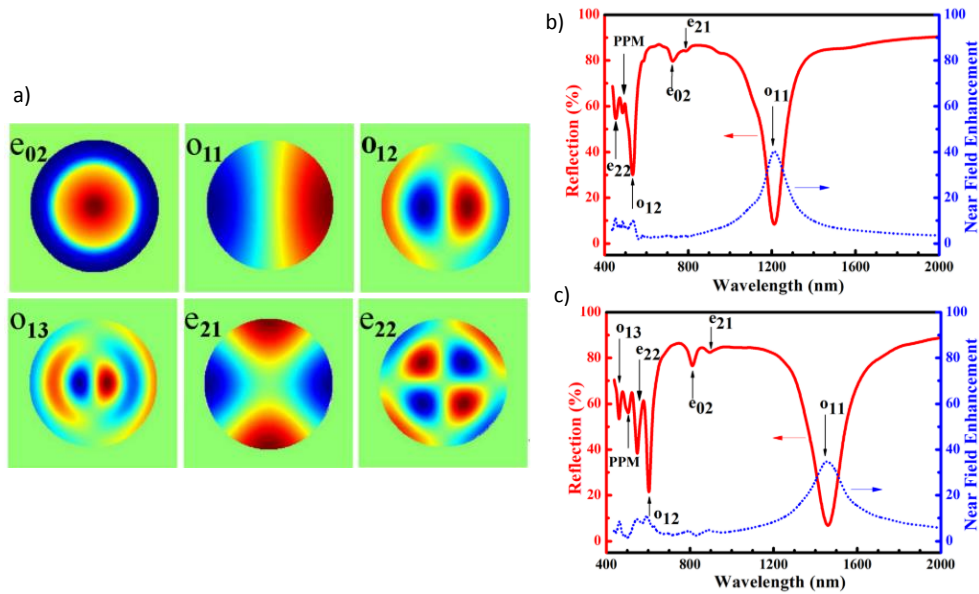
Figure 8: a) Simulation of modes existing in a cylindrical cavity at different resonance wavelengths. Simulation of reflectivity and amplification of electric field in the same cavities for arrays of period 500 nm and patch antenna diameter 100 nm (b) and 150 nm (c). Extracted from [38].
