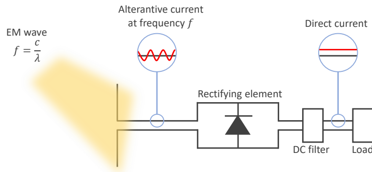
Figure 1: Scheme for the electronic operation of a rectifying antenna
