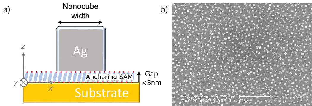
Figure 18: a) Concept of an optical rectifying antenna made of colloidal silver nanocube anchored with a SAM. Using anchoring molecules with rectification properties could lead to a rectenna device operating in the infrared or visible range, depending on the size of the nanoparticle and the length of the SAM. b) SEM image of an array of colloidal nanoantenna anchored with a thiolated SAM. Extracted from [66].
