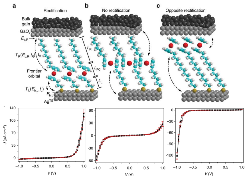
Figure 15: Diagram of SAM of ferrocene alkanethiol as a function of the position of the ferrocene moiety and associated current density - voltage characterisation a) Ferrocene at the bottom of the SAM b) Ferrocene in the middle of the SAM c) Ferrocène on the top of the SAM
