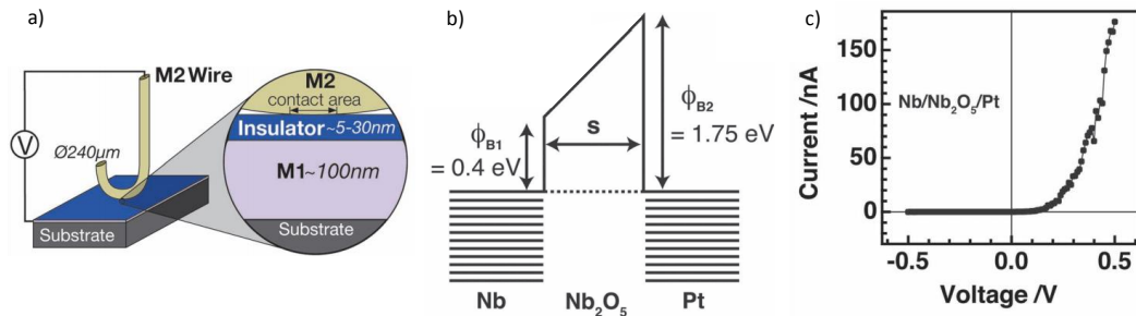
Figure 12: Exemples of MIM junctions. Extracted from [23] [47] and [48]
