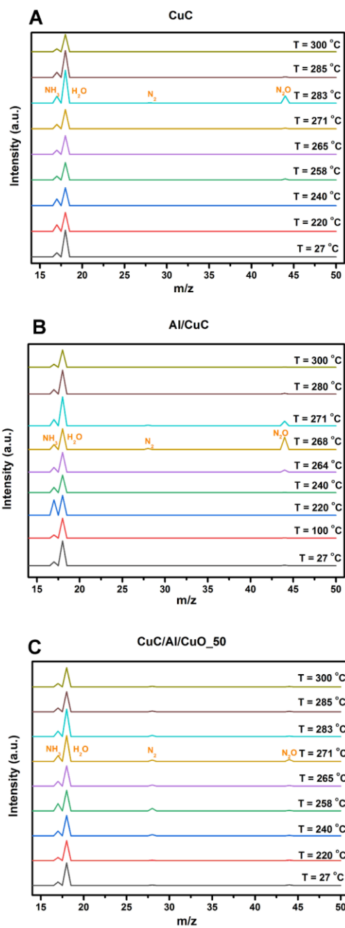
Figure 7. Mass spectra of CuC, Al/CuC and CuC/Al/CuO 50 energetic composites at various temperatures in argon environment.
