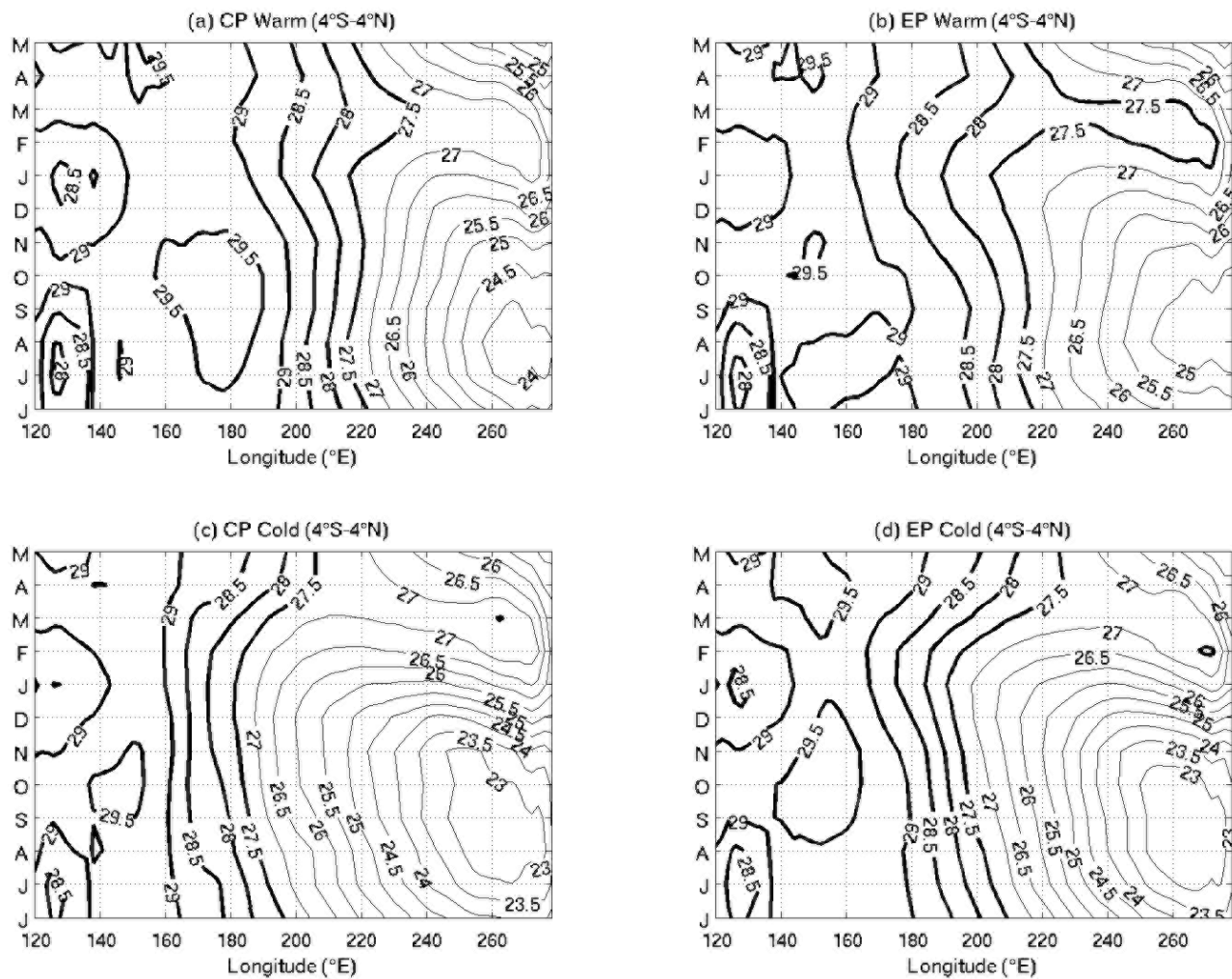
Figure 8. Time-longitude evolution of the SST averaged between 4^{\circ}\text{S} and 4^{\circ}\text{N} for the upper 15% percentiles of the (a) CP and (b) EP events and for the lower 15% percentiles of the (c) CP and (d) EP events defined from the SON season, from June to May of the following year.
