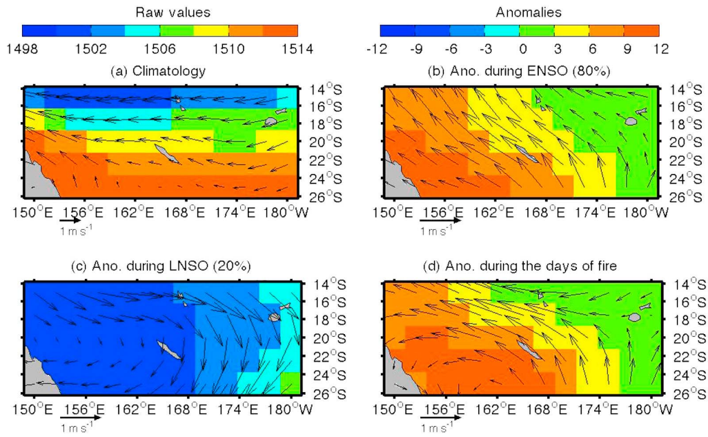
Figure 12. (a) Long-term mean (1950–2008) of winds (arrow) and geopotential height at 850 hPa (in m) in SON. Composite of seasonal anomalies in SON during the 12 (b) warmest and (c) coldest ENSO events. (d) Composite of daily anomalies during the days when at least one MODIS hotspot is recorded across NC.
