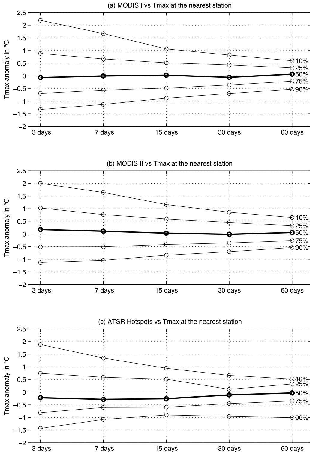
Figure 5. Percentiles (10%, 25%, 50%, 75%, 90%) of maximum temperature anomalies for 3 days, 7 days, 15 days, 30 days, and 60 days before (a) MODIS I, (b) MODIS II, and (c) ATSR hotspots at the closest meteorological station. The daily maximum temperatures are first averaged on running 3 day, 7 day, 15 day, 30 day, and 60 day windows, then normalized according to the 1996–2008 (2000–2008) climatology. The climatology is the daily mean low-pass filtered by a Butterworth recursive filter with a cutoff at 1/60 cycles per day.
