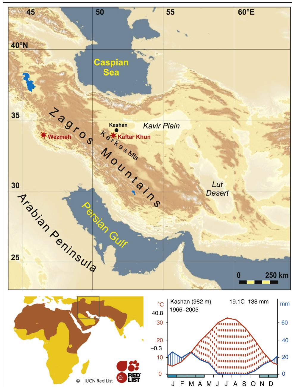
Fig. 1. a. Geographical position of the study site (Kaftar Khun) at the edge of central Iranian Plateau. b. The IUCN map for worldwide distribution of Hyaena hyaena (in dark brown) in Eurasia and Africa. c. Climate diagram based on Iran Meteorological Organization data from the city of Kashan. (For interpretation of the references to color in this figure legend, the reader is referred to the web version of this article.)
