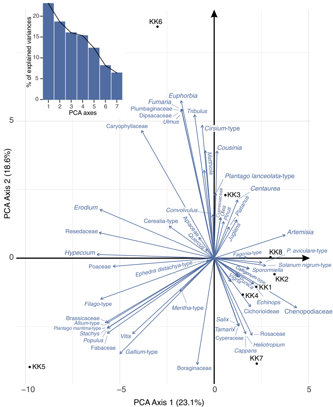
Fig. 5. PCA biplot comprising the main pollen types (variables) found in hyena scats K1 to K8 (samples).
