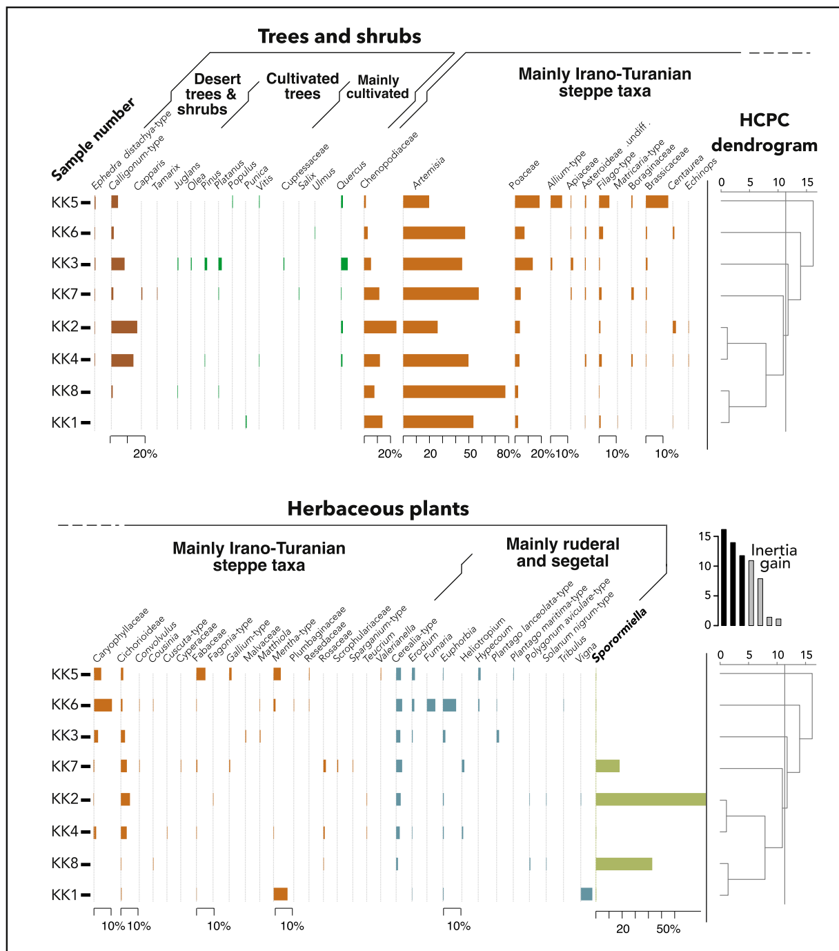
Fig. 4. Pollen percentage diagram of the eight hyena scats. Sporormiella percentage in sample KK2 is >2900% calculated based on total pollen sum.
