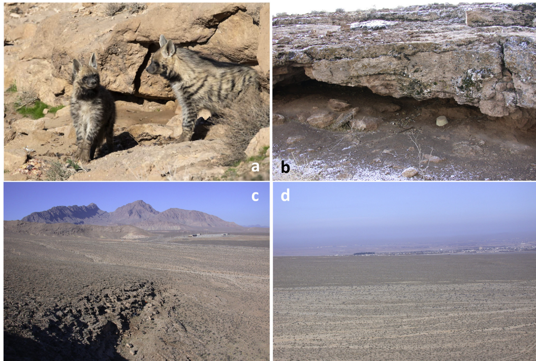
Fig. 2. a. Two striped hyenas recently photographed in central Iran (not Kaftar Khun). b. Den complexes are mostly found in rock shelters formed in limestone outcrops. c. The position of the den complex in a travertine outcrop, photo looking north. d. Photo looking northwest: foreground shows xerophytic desert Artemisia steppe and background shows the suburbs of the city of Kashan and the central Iranian desert. Photo a is courtesy of wildlife photographer M. Saeed Davari. Photos, b, c, and d by MM.
