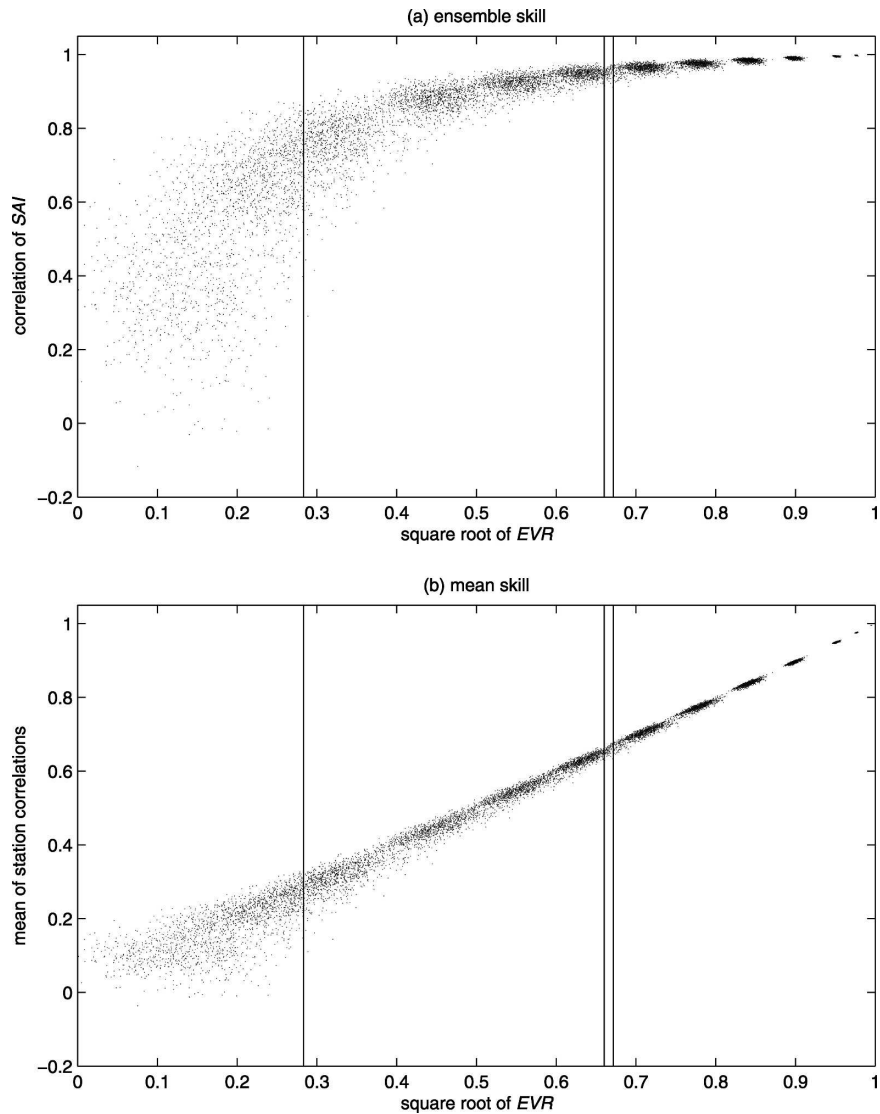
FIG. 5. Skill (temporal correlation between each column of \mathbf{X} and \mathbf{f} time series) vs the square root of EVR of \mathbf{X} for the 13 000 simulations of the random matrices of the same size as Senegal in case where \mathbf{X} = \mathbf{I}\mathbf{f} + \mathbf{N} . (a) Ensemble skill (temporal correlation between SAI of \mathbf{X} and \mathbf{f} ) and (b) mean skill (mean of the temporal correlation between each column of \mathbf{X} and \mathbf{f} ). The values are computed for an EVR of 1%, 5%, 10%, 20%, 30%, 40%, 50%, 60%, 70%, 80%, 90%, 95%, and 99%. The vertical lines indicate the empirical square root of EVR of seasonal amount, rainfall occurrence, and mean intensity (Table 1).
