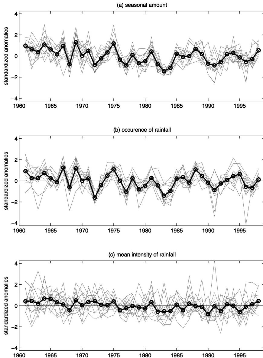
FIG. 3. Normalized anomalies of (a) seasonal amount, (b) rainfall occurrence, and (c) mean intensity of rainfall for the 13 stations of Senegal. The gray lines indicate each station and the boldface line with circles is the standardized anomaly index (= mean of the 13 stations).
