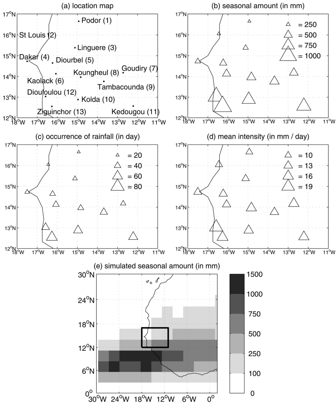
FIG. 1. (a) Location of the 13 stations used in this study; (b) seasonal amount (mm during JAS); (c) rainfall occurrence (number of rainy days receiving >0 mm); (d) daily mean intensity of rainfall ( \text{mm day}^{-1} ) during the wet day; and (e) seasonal amount (mm during JAS) for the 24-member ensemble of ECHAM 4.5. The black box represents the window used in other panels.
