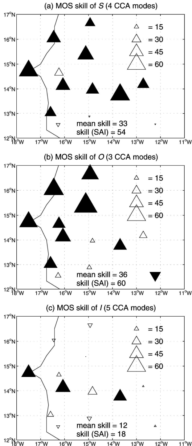
FIG. 8. Skill (= correlation \times 100 between observed and MOS corrected GCM time series) of (a) seasonal amount, (b) rainfall occurrence, and (c) daily mean intensity of rainfall. The MOS uses a cross-validated (5 yr are withheld at each turn) CCA between observed variables on the 13-station network and simulated variables from the 24-member within the region ( 0^{\circ} – 30^{\circ} N, 30^{\circ} W– 0^{\circ} ). The number of CCA modes included in the MOS correction is indicated in the title of each panel. Upper triangle indicates positive correlations and lower triangle indicates negative correlations. The filled triangles are significant at the two-sided 0.1 level according to a random-phase test (Janicot et al. 1996; Ebisuzaki 1997).
