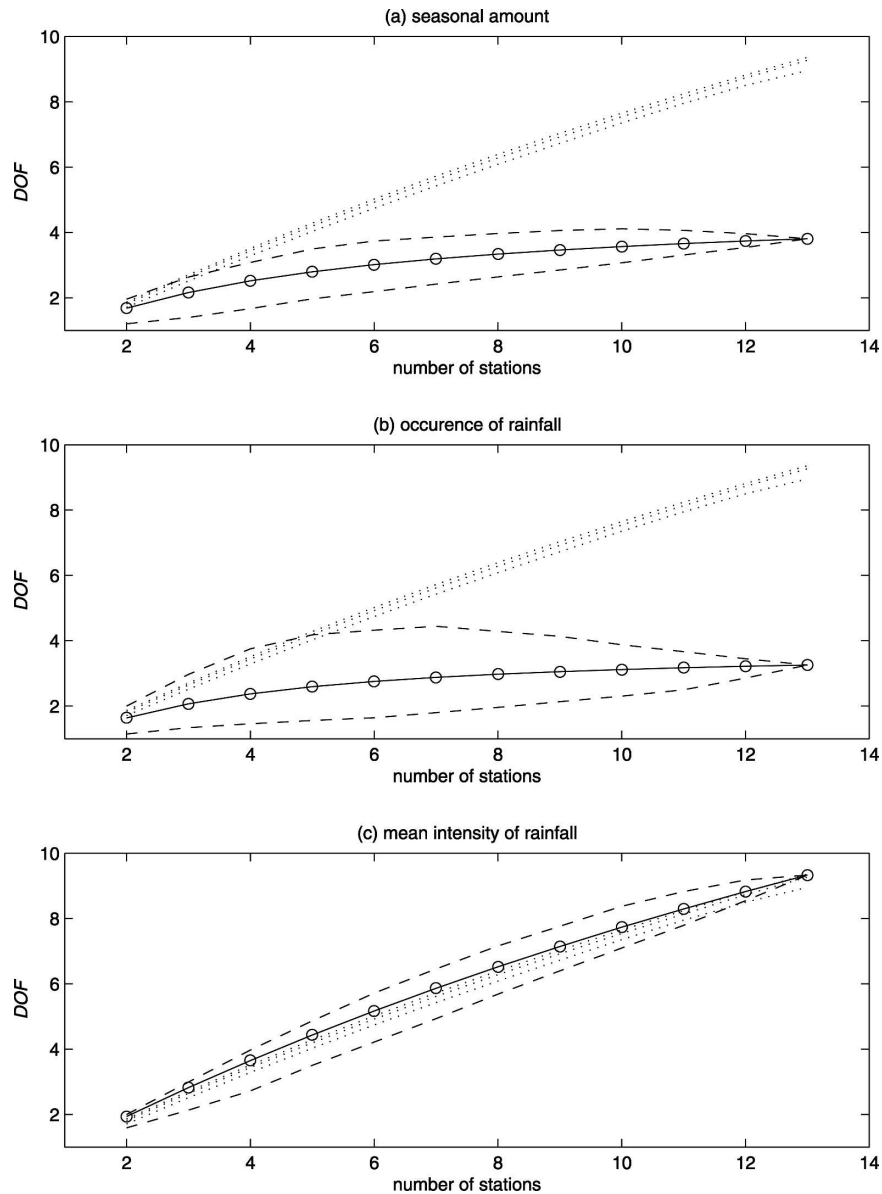
FIG. 4. Mean (solid line with circles) and minimum and maximum (dashed lines) of degrees of freedom (DOF) of all the combinations (from 2 to 13 stations) of (a) the seasonal amount, (b) rainfall occurrence, and (c) mean intensity of the 13 stations of the Senegal's network. There are 78, 286, 715, 1287, 1716, 1716, 1287, 715, 286, and 78, respectively, and 13 possible combinations of 2, 3, 4, 5, 6, 7, 8, 9, 10, 11, and 12 stations, respectively. The dotted lines give the 0.1, 0.05, and 0.01 levels of significance estimated from 100 random matrices of the same size as Senegal network (38 observations by 13 variables, which are independent from each other).
