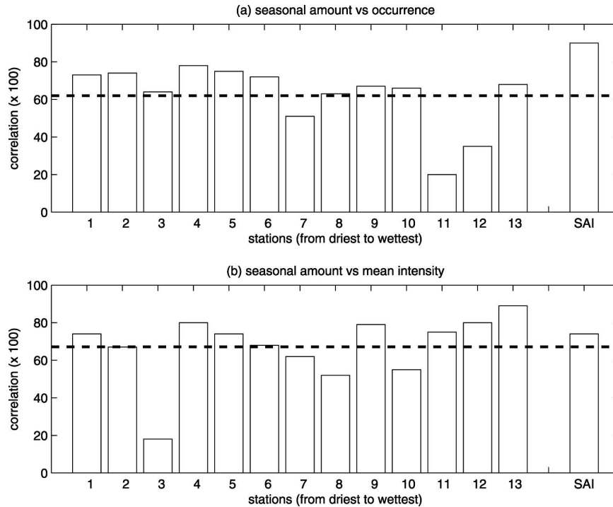
FIG. 2. Temporal correlation ( \times 100 ) (a) between seasonal amount and rainfall occurrence and (b) between seasonal amount and mean intensity for each station. The 13 stations are ranked from the driest to the wettest one (the numbers refer to Fig. 1a) and the last column gives the correlation between the SAI of (a) seasonal amount and rainfall occurrence and of (b) seasonal amount and mean intensity. The horizontal dashed line indicates the country average of the correlations between (a) seasonal amount and rainfall occurrence and (b) seasonal amount and mean intensity.
