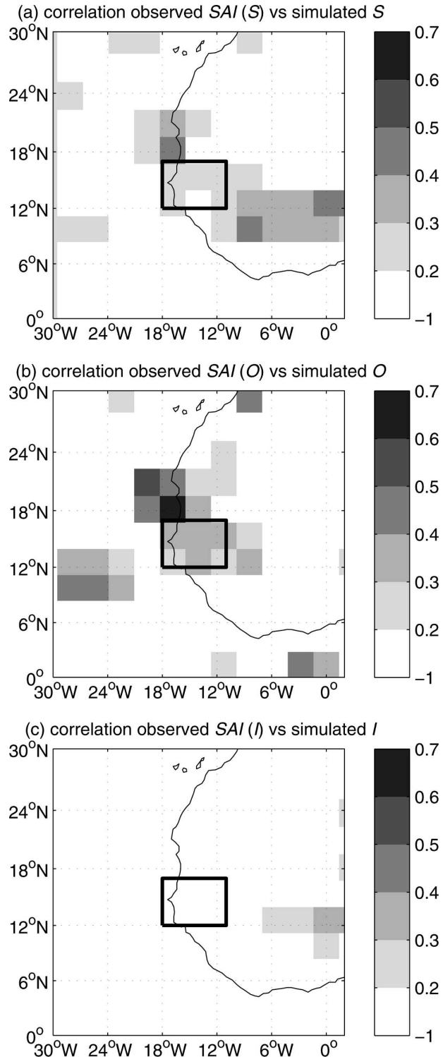
FIG. 7. Correlation between observed SAI (= country average of standardized anomalies) of (a) seasonal amount, (b) rainfall occurrence, (c) daily mean intensity of rainfall and the same quantities in the ensemble mean of ECHAM 4.5. In (b) and (c), the simulated occurrence and daily mean intensity of rainfall are computed only from simulated daily amounts >1 mm. The black box indicates the location of Senegal.
