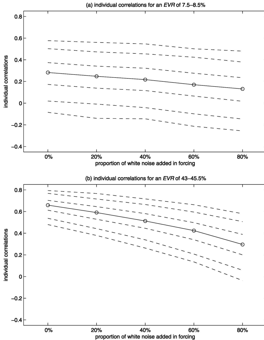
FIG. 6. Median (line with circles) and 1%, 5%, 25%, 75%, 95%, and 99% percentiles (dashed lines) of the individual skill (temporal correlations between each column of \mathbf{X} and \mathbf{f} time series) vs the amount of white noise ( \mathbf{v} ) added in \mathbf{f} in case, where \mathbf{X} = \mathbf{I}(\mathbf{f} + \mathbf{v}) + \mathbf{N} . One thousand random simulations are performed with \mathbf{v} accounting for 0%, 20%, 40%, 60%, and 80% of the temporal variance of (\mathbf{f} + \mathbf{v}) time series for an (a) EVR between 7.5% and 8.5% (typical of mean intensity of rainfall) and (b) EVR between 43% and 45.5% (typical of seasonal amount and rainfall occurrence).
