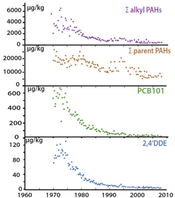
Fig. 4 Evolution of POP contamination in the Seine estuary sediment core EST (1970–2008) [26]
