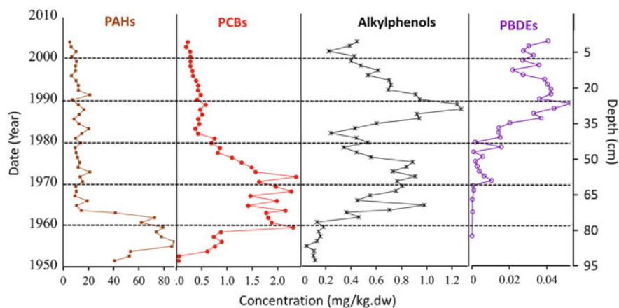
Fig. 3 POP contamination profiles ( \text{mg kg}^{-1} dry weight) for PAHs, PCBs, alkyl phenols and polybromodiphenylethers (PBDEs) in the Seine River floodplain core OUT 1 [15]
