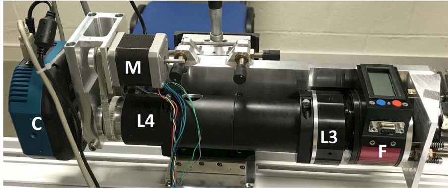
Fig. 2. The chamber of MeteoSpace H \alpha telescopes. L3 = chamber objective; F = DayStar Quantum PE Fabry P erot filter; L4 = field corrector/focuser; M = focuser motor; C = cooled CCD camera (QSI 660i).
