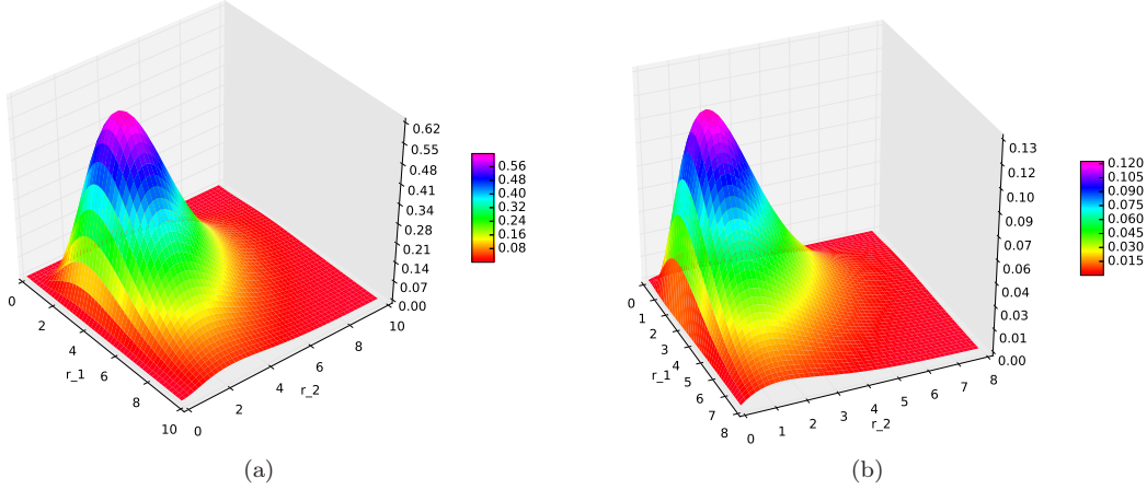
Figure 1: Shape of T_{(2,1)}^{(4)} (a) and T_{(2,1)}^{(4)}(r_1, r_2)/(r_1 r_2) (b), using the Laguerre function approximation scheme [25, Section 7.3].
