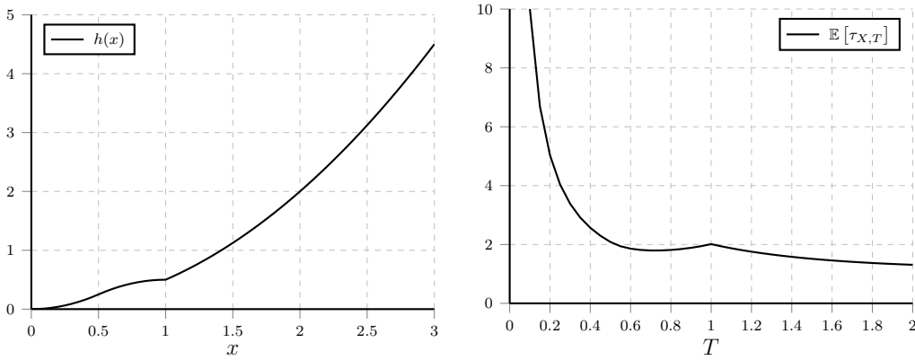
Figure 2: Plots of function h(x) (left) and the expectation \mathbb{E}[\tau_{X,T}] (right) as a function of T .
