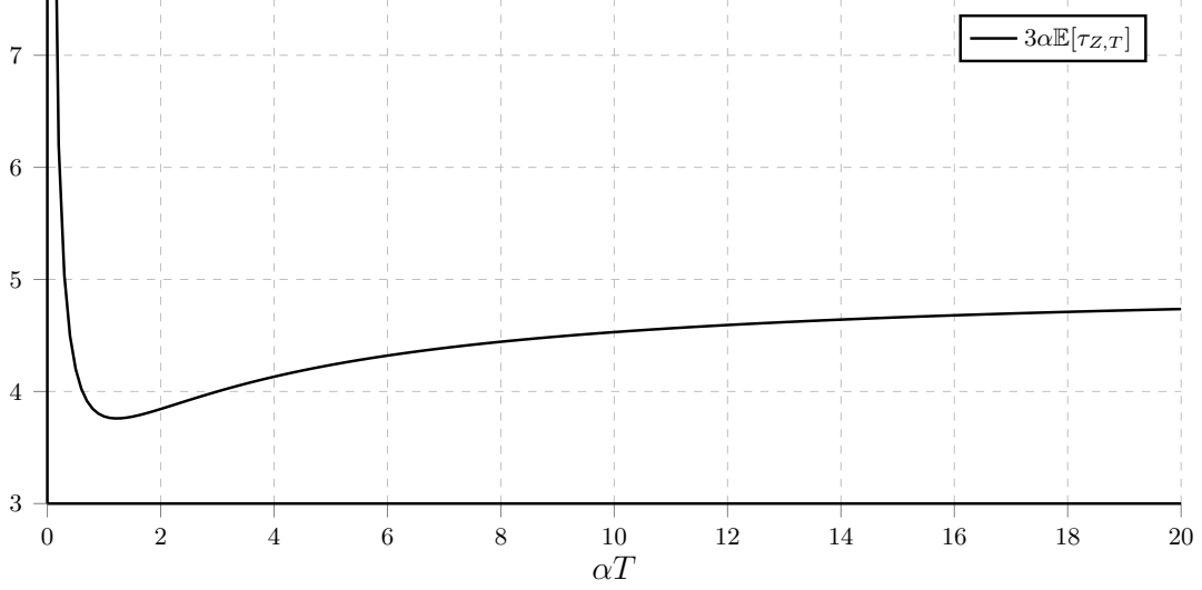
Figure 1: Plot of 3\alpha\mathbb{E}[\tau_{Z,T}] as a function of \alpha T .
