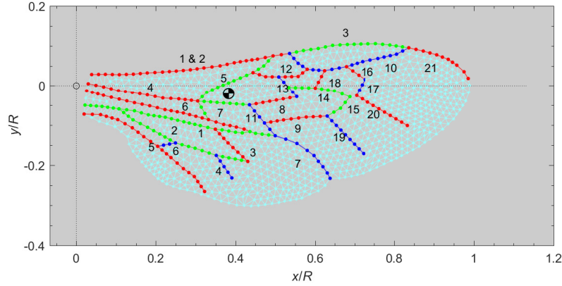
Fig. 3 Illustration of the mass-spring model which is meshed based on measured data of real bumblebee wings [26]. The black and white marker represents the mass center. Color codes (red, green and blue) are used for identifying the veins and the membranes are represented by cyan circles.
