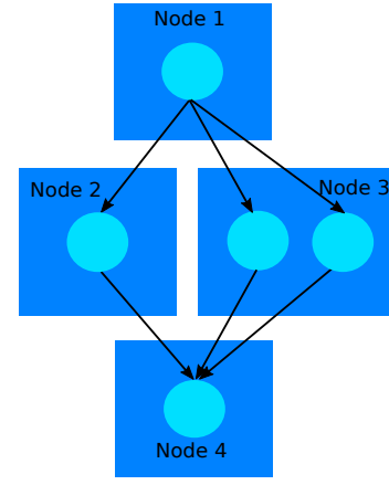
Fig. 1. Model parallelism
