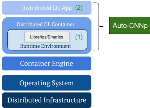
Fig. 4. Auto-CNNp operating scope: (1) runtime environment configuration and (2) user-specific deep learning execution schema definition.
