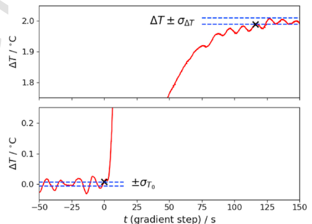
Fig. 9. Determining of the duration of the gradient build-up step (run 1r02).
