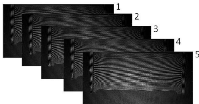
Fig. 2. The set of 5 fringes images for the 1_5_F691@0016_MN_DSC_190101_074147_5.stk file (run Sr01, cell #5, laser MN, Temperature gradient build-up step).
