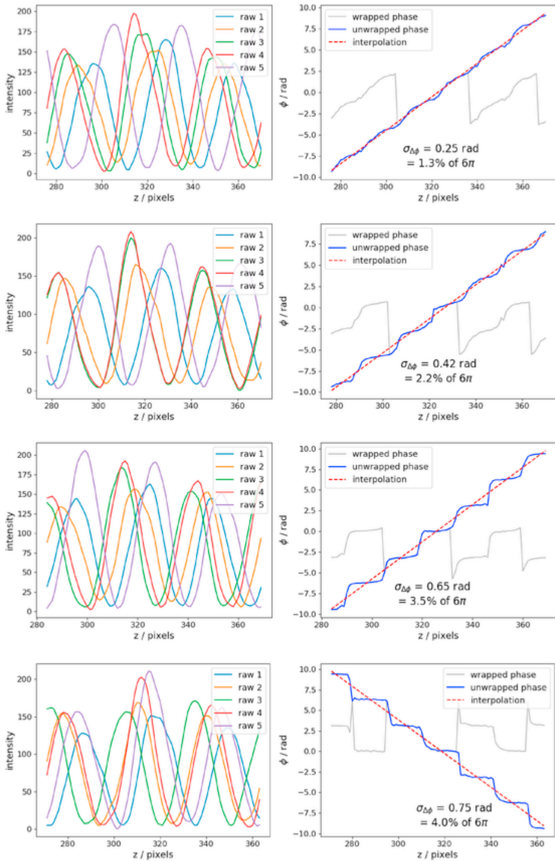
Fig. 6. Determining of the quality in the phase shift. Examples are taken from run 2r05, MR laser, Soret1 step, stacks #26, 30, 58 and 29 (from top to bottom).
