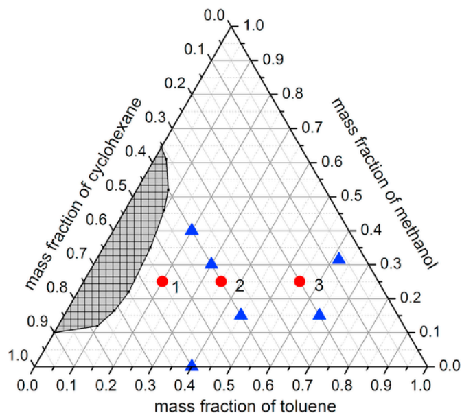
Fig. 1. Toluene-methanol-cyclohexane concentration diagram indicating DCMIX4 cells 1–3 composition (red circles) and as a reminder DCMIX2 samples composition (blue triangles). The hatched area indicates demixing zone at T = 25\text{ °C} ; the demixing zone expands as long as the temperature decrease. (For interpretation of the references to color in this figure legend, the reader is referred to the Web version of this article.)
