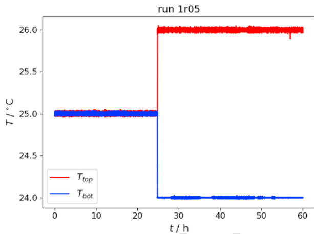
Fig. 8. Full temperature record of run 1r05.
