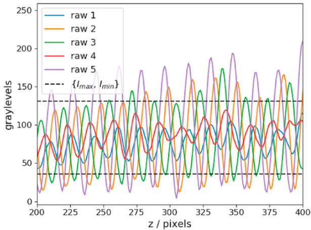
Fig. 5. Determining the contrast by all 5 fringe images of stack. I_{max} and I_{min} graylevels are obtained by averaging over the plotted vertical intensity profiles. The raw data are taken from the same stack as in Fig. 4.
