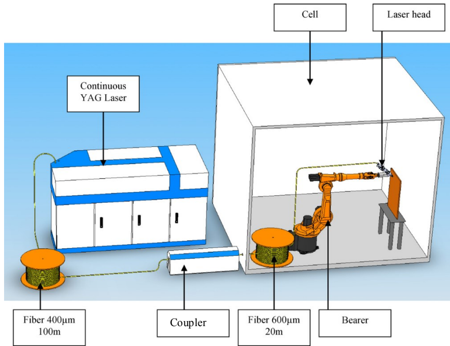
Figure 4 : Sketch of the laser cutting installation in the DELIA facility in a case of in air cutting site (aerosol generation part- (Figure 1 Chagnot et al [19]). The cutting cell is a stainless tank (1.38 m in diameter and 3 m length, 3.7 m 3 usable volume, 5 m 3 with chimneys).
