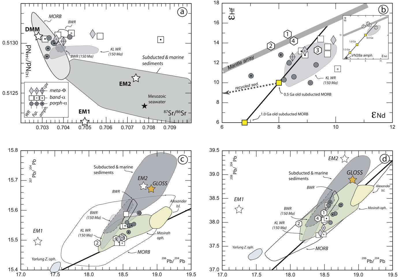
Fig. 9. Initial Sr-Nd-Hf-Pb isotope correlation diagrams for Kef Lakhal amphibolites and metagabbros. The field KL WR 150 refers to the isotopic ratios corrected for t = 150 Ma (Kef Lakhal Whole-rock 150 Ma). The fields BWR and BWR (150 Ma) refer to Kef Lakhal whole-rock analyses quoted in Bosch et al. (2014), age-corrected at 40 Ma and 150 Ma, respectively. (a) ^{143}\text{Nd}/^{144}\text{Nd} vs ^{87}\text{Sr}/^{86}\text{Sr} diagram; (b) ^{176}\text{Hf}/^{177}\text{Hf} vs ^{143}\text{Nd}/^{144}\text{Nd} diagram. The mantle array ( \epsilon\text{Hf} = 1.33 \times \epsilon\text{Nd} + 3.19 ) is from Vervoort et al. (1999). Old recycled oceanic crust (yellow squares) and associated sediments (grey dashed arrow) are from Geldmacher et al. (2011); (c) ^{207}\text{Pb}/^{204}\text{Pb} vs ^{206}\text{Pb}/^{204}\text{Pb} diagram; (d) ^{208}\text{Pb}/^{204}\text{Pb} vs ^{206}\text{Pb}/^{204}\text{Pb} diagram. Reported for comparison are: subducted and marine sediments (Ben Othman et al., 1989; Plank and Langmuir, 1998; Vervoort et al., 2011). DMM (Depleted MORB Mantle; Workman and Hart, 2005), EM1, and EM2 (Enriched Mantle Type-1 and Type-2; Hart, 1988), and GLOSS (Global Subducting Sediments; Plank and Langmuir, 1998). MORB field from Georoc database http://georoc.mpch-mainz.gwdg.de/georoc/ . Fields for Yarlung Zangpo ophiolite (Southern Tibet), Masirah ophiolite (Oman) and Alexander Island ophiolite (Antarctica) are from Mahoney et al. (1998). Symbols as follow: squares, grey circles, and grey diamonds are bulk rock analyses for banded amphibolites, porphyroblastic amphibolites and metagabbros respectively. Black dot, white dot and cross within symbols indicate mineral fraction analyses for amphibole, feldspar and pyroxene respectively. Empty hexagons labelled 1, 2, 3 and 4 are Atlantic, Pacific, Indian (White and Klein, 2014) and Global (Arevalo and McDonough, 2010) MORB. (For interpretation of the references to colour in this figure legend, the reader is referred to the web version of this article.)
