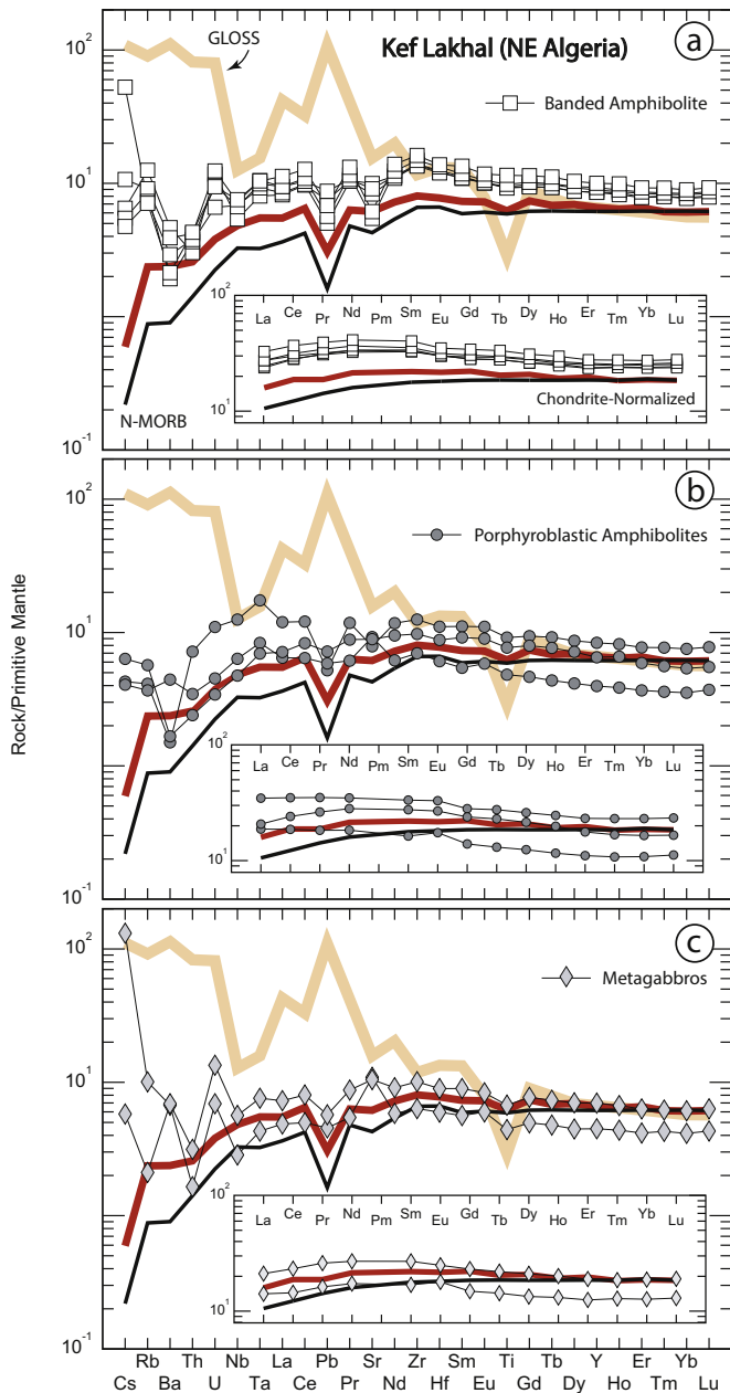
Fig. 7. Primitive mantle-normalized multi-elemental and chondrite-normalized REE diagrams for Kef Lakkhal amphibolites and metagabbros. The thick red line is Global MORB (Arevalo and McDonough, 2010). N-MORB (plain black line) and normalization values (Primitive Mantle and Chondrite) are from Sun and McDonough (1989). (For interpretation of the references to colour in this figure legend, the reader is referred to the web version of this article.)
