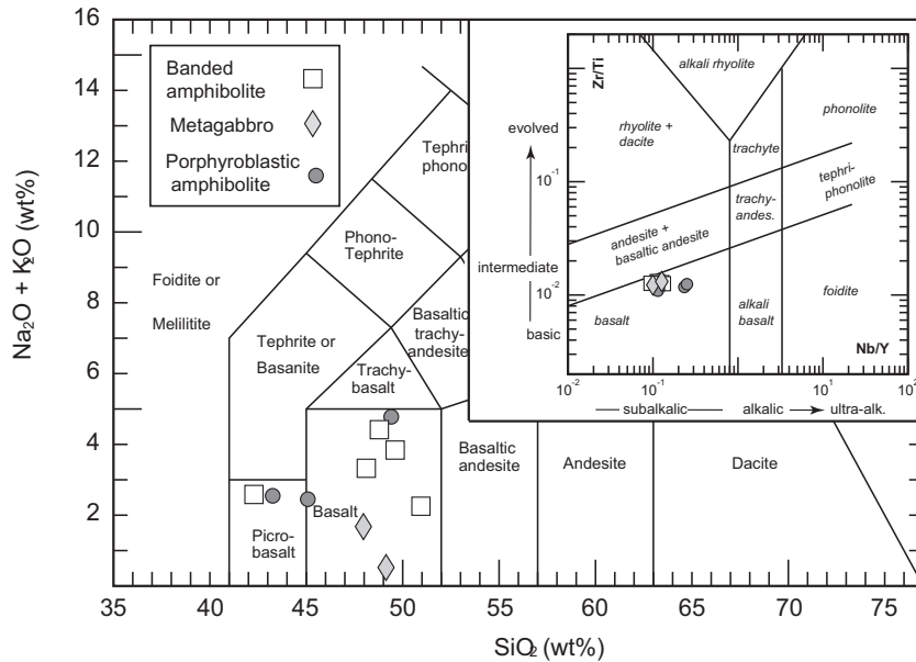
Fig. 6. TAS (Total Alkali Silica) diagram after Le Bas et al. (1986) and Zr/Ti vs. Nb/Y discrimination diagram for immobile elements of Pearce (1996).
