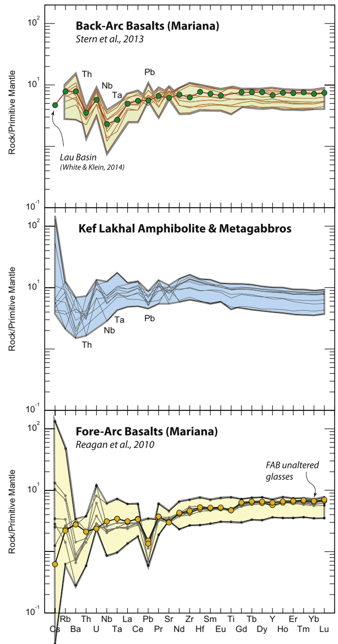
Fig. 14. Comparison of back-arc basalts (Stern et al., 2013) and fore-arc basalts (Reagan et al., 2010) from the Mariana and the Kef Lakhal samples. The spectrum of the Lau back-arc basin basalts is from White and Klein (2014). Note that, conversely to BABB, the Kef Lakhal samples do not show Nb—Ta negative anomalies, nor Pb positive spikes. LILE enrichments (Rb, Cs \pm Ba) and U spikes are related to seawater alteration and not to addition of a subduction component.
