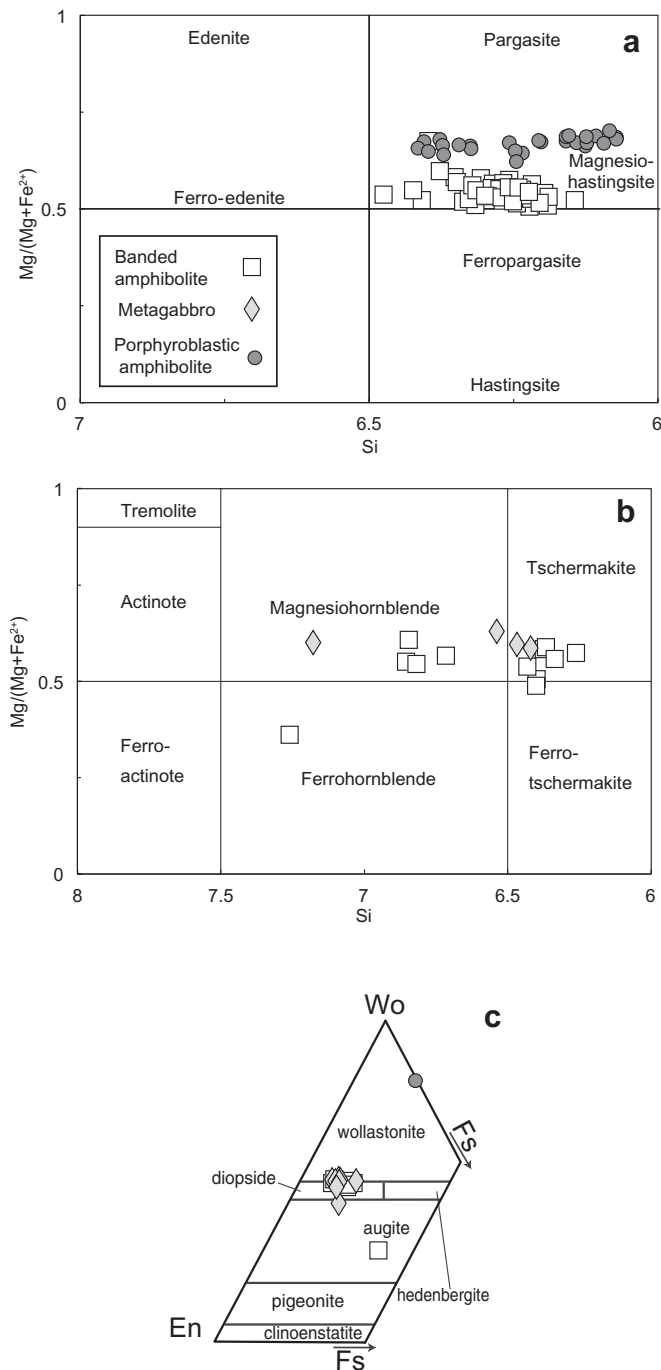
Fig. 5. Discriminant diagrams for amphibole after Leake et al. (1997) calculated in atom per formula unit. a) Calcic amphibole with: Ca_B > 1.50 ; (Na + K)_A > 0.50 ; Ti < 0.50 . b) For calcic amphibole satisfying the following criteria: Ca_B \geq 1.50 ; (Na + K)_A < 0.50 ; Ca_A < 0.50 . c) Ternary diagram for major elements in situ analyses of pyroxene (Morimoto, 1988). Abbreviations: (Wo) Wollastonite, (En) Enstatite, (Fs) Forsterite.
