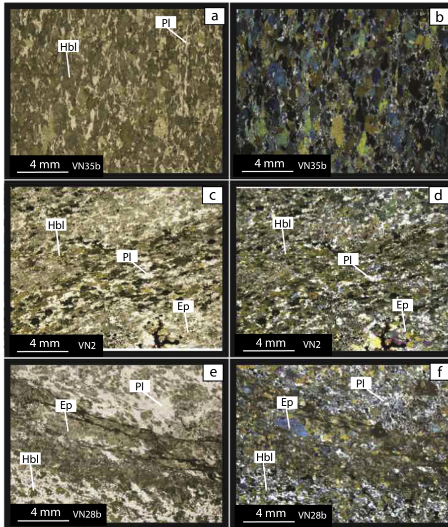
Fig. 3. Representative thin section microphotographs of Kef Lakhal amphibolites and metagabbros. a-b) amphibolite VN35b with hornblende porphyroblast and finely crystallized plagioclase and quartz; c-d) amphibolite VN2 with oxide-rich epidote levels; e-f) metagabbro VN28b rich in epidote, with some levels containing plagioclase, quartz and hornblende. Abbreviations are the followings: Pl: plagioclase, Ep: epidote, Hbl: hornblende.
