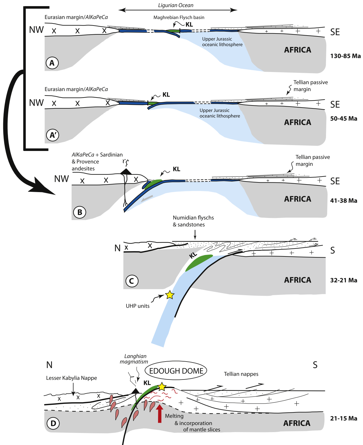
Fig. 15. Cartoon showing the scenario for the origin of the Kef Lakhal Complex in the context of the Western Mediterranean. Stages A and A' correspond to the two alternative possibilities for initiation of the Kef Lakhal fore-arc, either Cretaceous, or Middle Eocene. Stage A represents the East directed intra-oceanic subduction of the western part of the Ligurian Ocean occurring between 130 Ma and 85 Ma ( Handy et al., 2010 ). Stage A' represents a flip of the subduction with the northwestward-directed subduction of the remnant of the Ligurian Ocean below the Iberia-Eurasia/AlKaPeCa margin taking place at around 45 Ma onward ( Carminati et al., 2012 ). In the proposed scenario, this first stage (A or A') is followed by steps B, C and D. See text for explanation. KL stands for Kef Lakhal.
