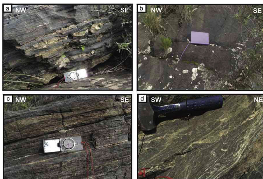
Fig. 2. Field pictures showing different types of amphibolites. a-b) Amphibolite from the top of the Kef Lakhel complex mainly composed of feldspar and amphibole and showing deformed epidote-rich levels. c) Amphibolite with plagioclase-rich levels. d) Traces of partial melting in this amphibolite.
