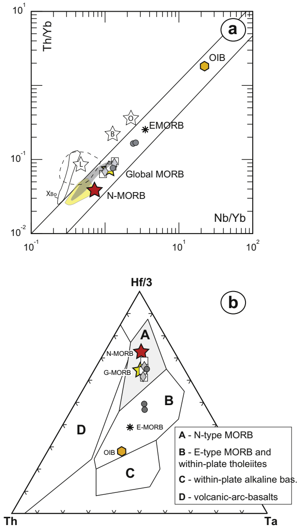
Fig. 10. (a) Th/Yb vs. Nb/Yb diagram (Pearce, 2008). N-MORB, E-MORB and OIB after Sun and McDonough (1989). Global MORB after Arevalo and McDonough (2010). Stars labelled B, L, and O are back-arc basin basalts: Global back-arc basin, Lau basin, and Okinawa Trough respectively (White and Klein, 2014). The grey field and yellow field are fore-arc basalts from the Mariana (Reagan et al., 2010) and Xigaze ophiolite (Dai et al., 2013), respectively. The empty dashed domain is back-arc basin basalts from the Mariana (Stern et al., 2013). XBo is the field of boninite from the Xigaze ophiolite (Dai et al., 2013). (b) Hf/3-Th-Ta ternary diagram (Wood, 1980). (For interpretation of the references to colour in this figure legend, the reader is referred to the web version of this article.)
