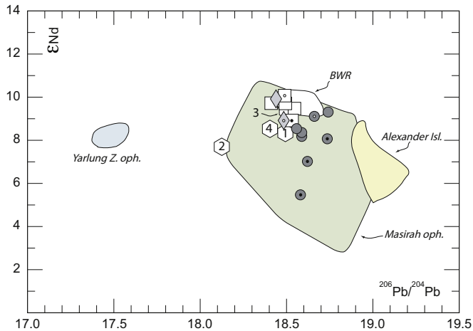
Fig. 12. \epsilon_{\text{Nd}} vs. ^{206}\text{Pb}/^{204}\text{Pb} diagram. Empty hexagons labelled 1, 2, 3 and 4 correspond to Atlantic, Indian, Pacific (White and Klein, 2014) and Global MORB (Arealo and McDonough, 2010) respectively. The fields for Masirah, Alexander Island (Atlantic/Pacific Tethyan ophiolites) and Yarlung Zangpo (Indian-type Tethyan ophiolite) are from Mahoney et al. (1998). The field BWR refers to Kef Lakhal whole-rock analyses quoted in Bosch et al. (2014), age-corrected at 40 Ma.
