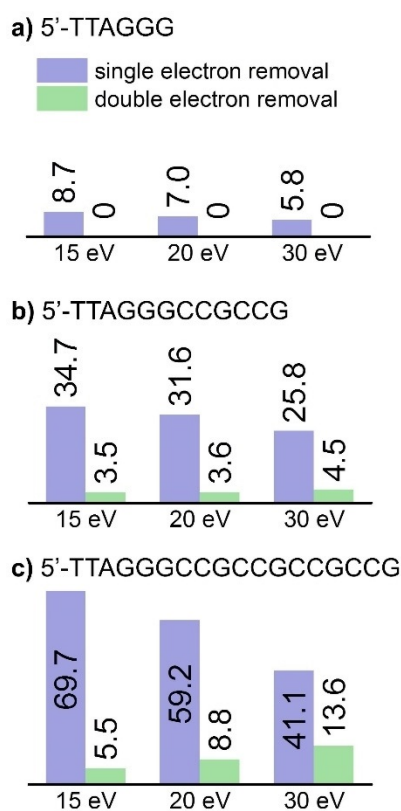
Figure 2. Single electron removal (blue) and double electron removal (green) yields in percent of the precursor ion loss for the deprotonated oligonucleotides ( dTTAGGG-3H ) 3- (a), ( dTTAGGG(CCG)_2-5H ) 5- (b) and ( dTTAGGG(CCG)_4-7H ) 7- (c) for three photon energies.
