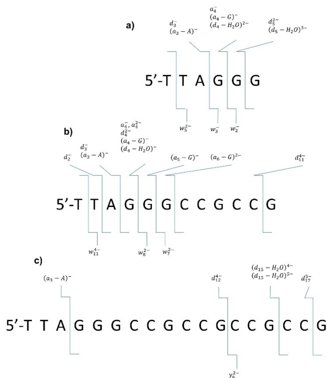
Figure 3. Fragments observed for VUV photofragmentation of ( dTTAGGG-3H ) 3- , ( dTTAGGG(CCG)_2-5H ) 5- and ( dTTAGGG(CCG)_4-7H ) 7- . Fragments given above the respective sequence are from the 5'-side (left), fragments below are from the 3'-side (right).
