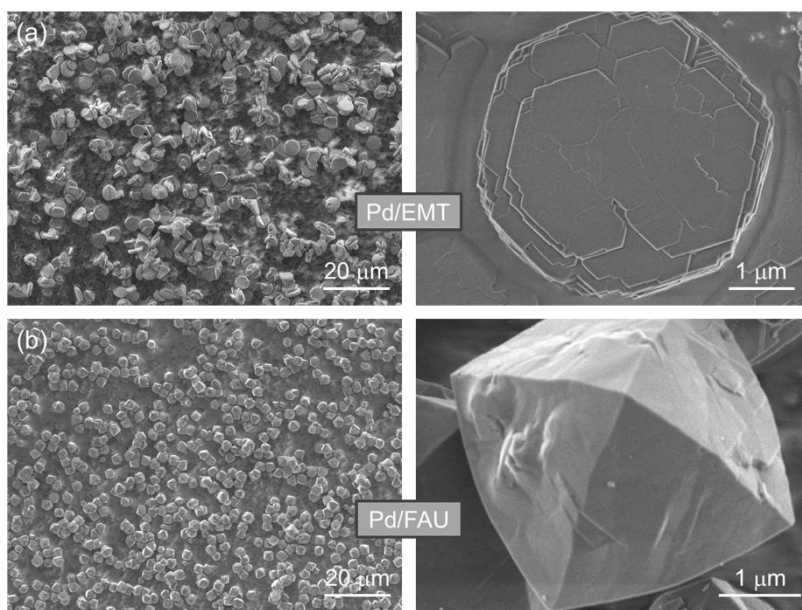
Fig. 1. SEM images of the (a) Pd/EMT and (b) Pd/FAU catalysts.
