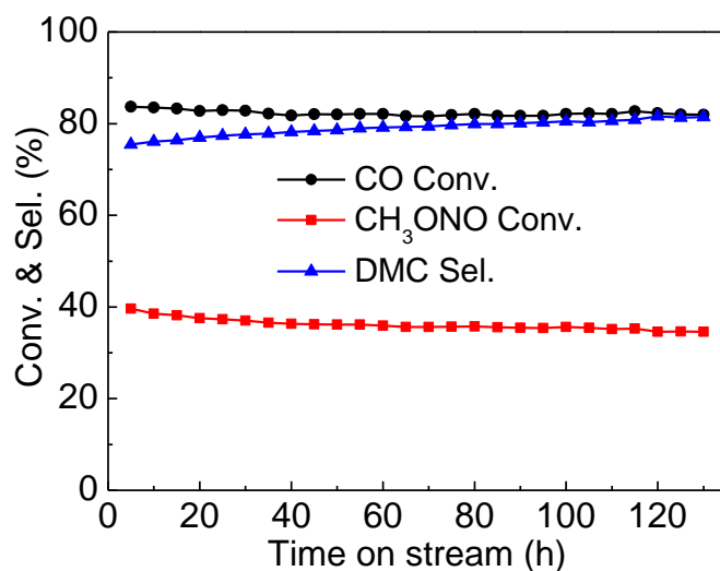
Fig. 12. Durability performance of the Pd/EMT catalyst in the indirect oxidative carbonylation of methanol to DMC measured for 130 h. Reaction conditions: 0.1000 g catalyst, \text{CO}/\text{CH}_3\text{ONO}/\text{N}_2 = 1/6/33 (volume), \text{GHSV} = 8,000 \text{ mL g}^{-1} \text{ h}^{-1} , 110 \text{ }^\circ\text{C} , 0.1 \text{ MPa} . For each point an average of 3 measurements was conducted.
