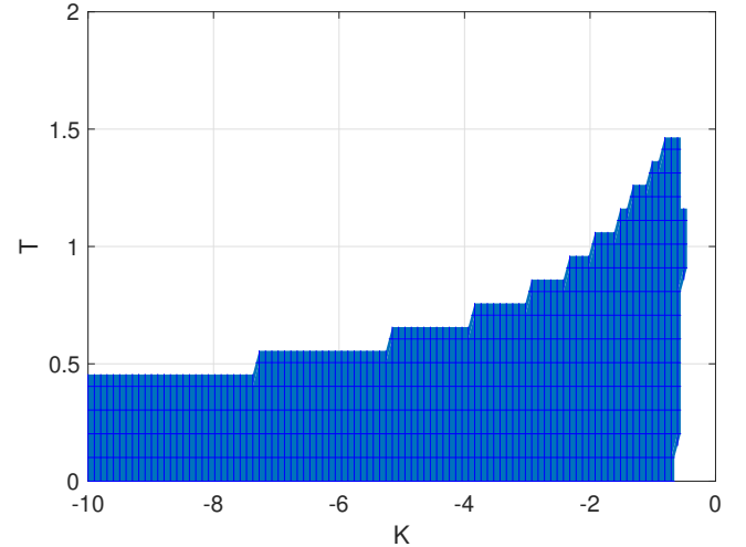
Fig. 2. Feasible region of the pair K, T where the satisfied conditions for global exponential stability are satisfied when H = 0.5
