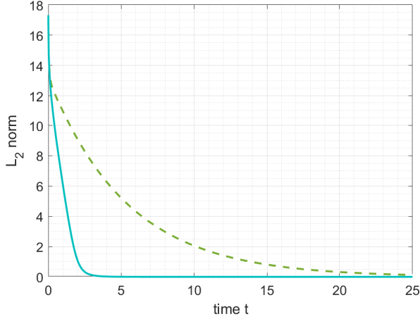
Fig. 4. Case 1: The time evolution of the spatial norm \mathcal{L}_2 of X(t, \cdot) in closed-loop (solid-line) and open-loop (dashed-line)
