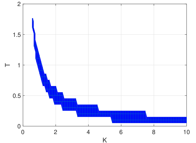
Fig. 3. Feasible region of the pair K, T where the satisfied conditions for global exponential stability are satisfied when H = -0.99
