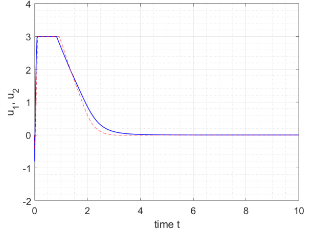
Fig. 5. Time evolution of \sigma_1(K_1X_1(t,1)) (solid-line) and \sigma_2(K_2X_2(t,1)) (dashed-line) with respect to time for Case 2
