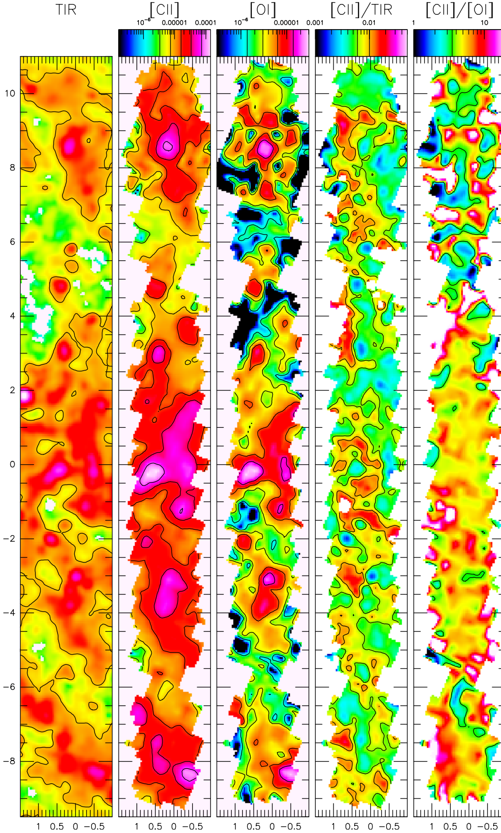
Fig. 2. Central part of the PACS maps of M33. From left to right: intensities of total infrared continuum (TIR), [C II], [O I](63 μm), [C II]/TIR, and [C II]/[O I] intensity ratios. Intensities are in units of \text{erg s}^{-1} \text{cm}^{-2} \text{sr}^{-1} . Offsets are in arcminutes relative to the nucleus, after de-rotation of the position angle by 22.5^\circ . The TIR contour is at 2 \times 10^{-3} \text{erg s}^{-1} \text{cm}^{-2} \text{sr}^{-1} , the threshold intensity used in the correlation plots to distinguish TIR-bright and TIR-weak regions (Figs. 4–6, 8, 5). The color wedge is the same as in Fig. 1. [C II] contours are the same as in Fig. 1. [O I] contours are 1.4, 3.0, 6.3, 13.8 in units of 10^{-6} \text{erg s}^{-1} \text{cm}^{-2} \text{sr}^{-1} . The map of [C II]/TIR is overlaid with contours at the 0.6% and 1% level of the ratio. The map of [C II]/[O I] is overlaid with the contour of 3.5. Long tic marks in the color wedges indicate contour levels.
