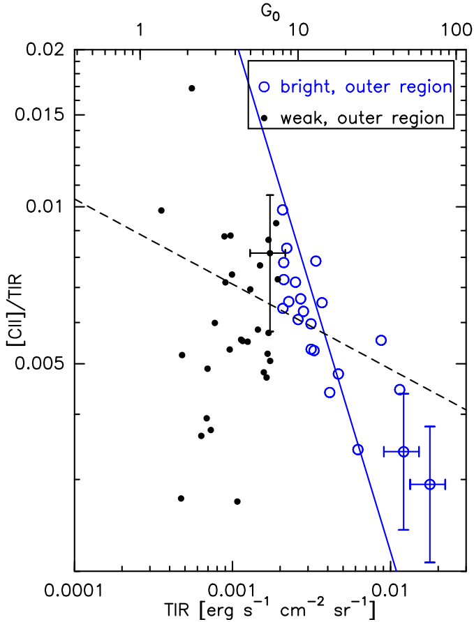
Fig. 9. [C II]/TIR intensity ratio versus TIR for the northern H II region BCLMP 691 in M 33. The blue drawn line shows the result of an unweighted linear least-squares fit to the TIR-bright data of BCLMP 691 varying only the y-intercept, while keeping the slope fixed at -1 . The black dashed line shows the result of an unweighted linear least-squares fit to all M 33 data (cf. Fig. 5). A few typical 1\sigma errorbars are shown.
