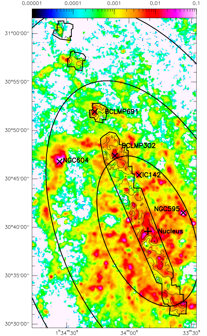
Fig. 1. M 33 map of the total far-infrared (TIR) continuum in color together with [C\text{II}] contours, both at 12'' resolution. TIR units are \text{erg s}^{-1} \text{cm}^{-2} \text{sr}^{-1} . [C\text{II}] contours are 3.4, 7.4, 16.0, 33.6, 73.0 in units of 10^{-6} \text{erg s}^{-1} \text{cm}^{-2} \text{sr}^{-1} . A polygon marks the outer edges of the regions mapped in [C\text{II}] . Coordinates are in RA and Dec (eq. J2000). The nucleus at 1:33:50.9 , 30:39:35.8 (J2000) ( Skrutskie et al. 2006 ) is marked, together with a few prominent giant H II regions. Ellipses delineate galacto-centric distances of 2, 4, and 6 kpc.
