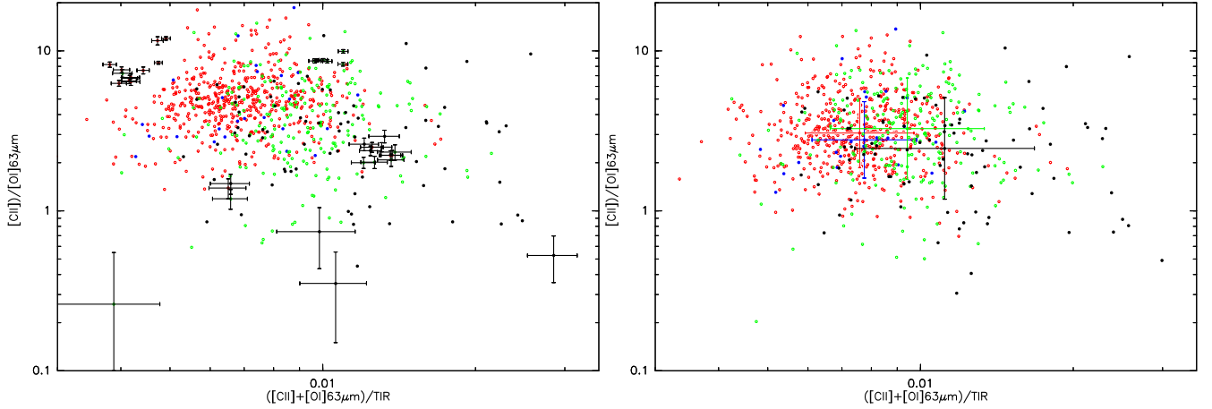
Fig. 7. [\text{C II}]/[\text{O I}](63\ \mu\text{m}) ratio plotted against the ([\text{C II}]+[\text{O I}](63\ \mu\text{m}))/\text{TIR} ratio for M33. [\text{C II}] , [\text{O I}] , and TIR intensities are from positions with intensities above the local 3\sigma value. Colors correspond to the four different regions of the inner and outer galaxy, and above and below a TIR threshold, as described in Sect. 3.1. Left: observed ratios with typical 1\sigma errors. Right: ratios with corrected [\text{O I}] intensities, as described in Sect. 3.2.4. In addition, median and standard deviations are shown for the four regions (errorbars in color) (cf. Table 5).
