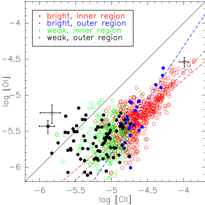
Fig. 6. Observed intensities of [O I](63 \mu m) and [C II] in M33 with representative 1\sigma errorbars. The straight black line corresponds to a ratio of 1. The dashed black line corresponds to the average [C II]/[O I] ratio (Table 5). The red and blue dashed lines are the results of unweighted least squares fits to the TIR-bright inner and outer regions, respectively (Table 4).
