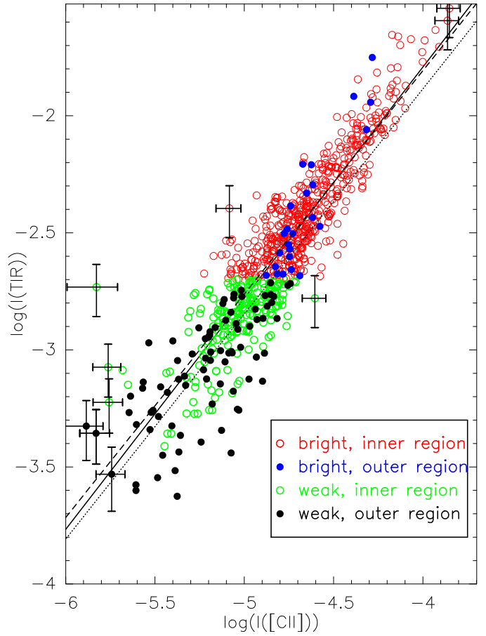
Fig. 4. Total infrared continuum intensity (TIR) versus [C II] intensities in M 33. Intensities are given in \text{erg s}^{-1}\ \text{cm}^{-2}\ \text{sr}^{-1} . Each point corresponds to one position on a 12'' grid at 12'' resolution, with an intensity 3 times above the local rms, for [C II], [O I], and TIR. Typical 1\sigma errorbars are shown. Colors correspond to the four different regions of the inner and outer galaxy, and above and below a TIR threshold, as described in Sect. 3.1. Straight lines delineate the results of unweighted linear least-squares fits to all data (drawn), the inner galaxy (dashed), and the outer galaxy (dotted) (Table 1).
