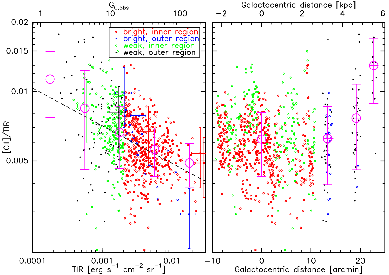
Fig. 5. Left: [\text{C II}]/\text{TIR} intensity ratio versus TIR and corresponding FUV field G_{0,\text{obs}} in M33 (see Eq. (2) in Sect. 3.1). The large pink points and errorbars show binned ratios (Table 2). Errorbars represent the standard deviation of the data. The dashed line shows the result of an unweighted least-squares fit to \log([\text{C II}]/\text{TIR}) = b + m \times \log \text{TIR} and all ratios, which gives m = -0.16 \pm 0.10 and b = -2.64 \pm 0.26 , with correlation coefficient r = -0.39 . For a few of the individual points 1\sigma errorbars are shown. Right: [\text{C II}]/\text{TIR} versus projected galacto-centric radius in M33. The large pink points and errorbars show ratios binned over selected ranges of radii (Table 3).
