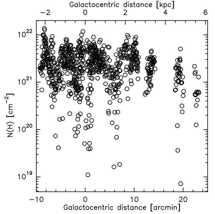
Fig. B.4. Total hydrogen column densities derived from fits of modified black bodies to the 70\ \mu\text{m} , 100\ \mu\text{m} , and 160\ \mu\text{m} data at each position, assuming a constant gas-to-dust ratio (see Sect. 3.2.4).
