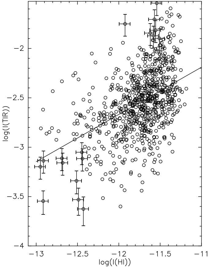
Fig. B.3. TIR versus HI intensities in M33. Intensities are given in \text{erg s}^{-1} \text{cm}^{-2} \text{sr}^{-1} . Typical 1\sigma errorbars are shown. For HI we assume an calibration error of 15% (cf. K2013). The drawn line shows the result of an unweighted linear least-squares fit to \log \text{TIR} = b + m \times \log \text{HI} , which gives a slope m = 0.48 \pm 0.11 , y-intercept b = 3.07 \pm 1.32 , and correlation coefficient r = 0.45 .
