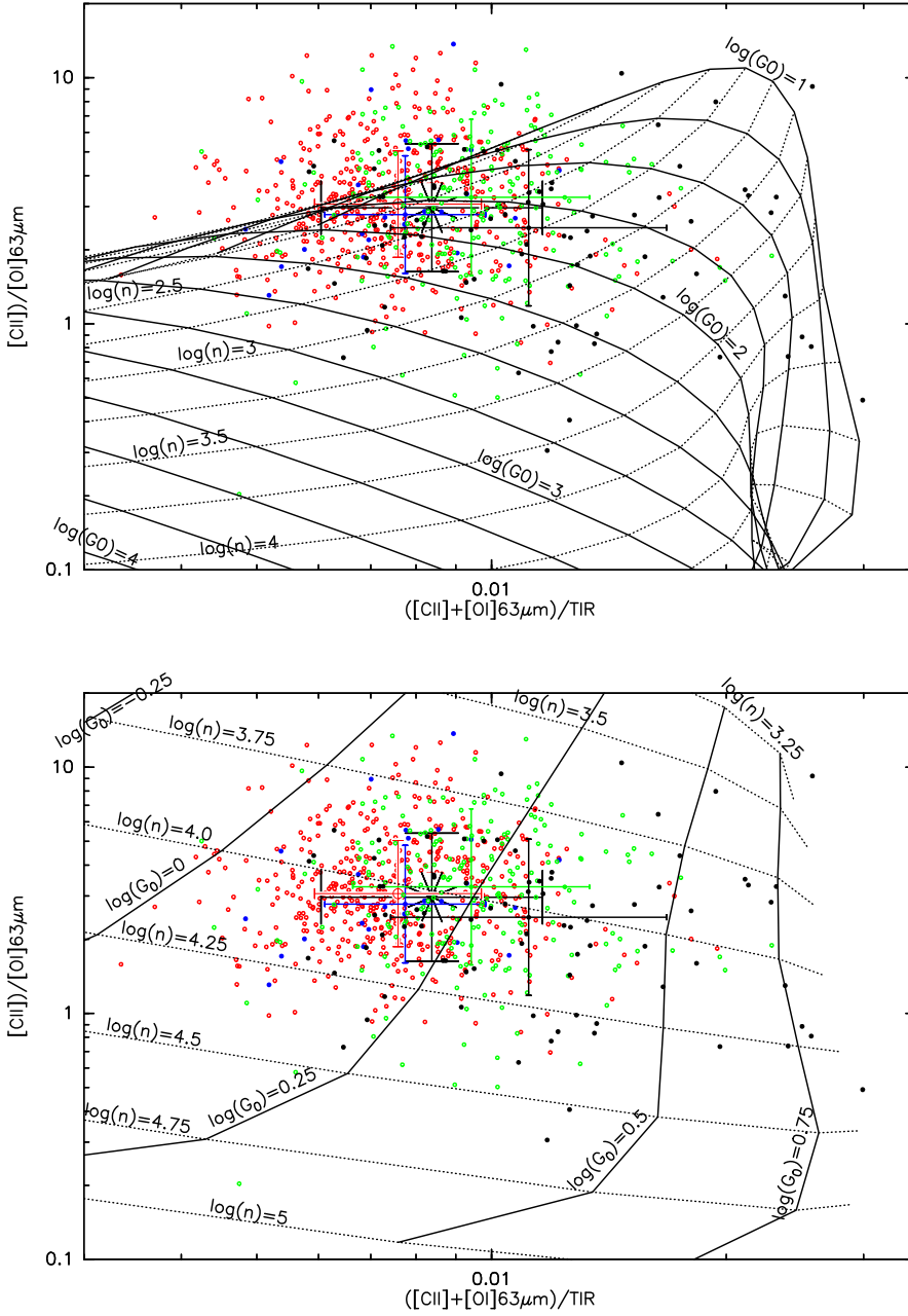
Fig. 8. Diagnostic diagram of the [\text{C II}]/[\text{O I}] ( 63\ \mu\text{m} ) ratio plotted against the ([\text{C II}]+[\text{O I}]) ( 63\ \mu\text{m} )/TIR ratio for M33, using the corrected [\text{O I}] intensities (see Sect. 3.2.4). Median and standard deviation of the four regions are shown in color, and of all data (star and large errorbars). Colors correspond to the four different regions as described in Sect. 3.1: the TIR bright, inner region (red), the bright, outer region (blue), the weak, inner region (green), and the weak, outer region (black). Superimposed is a grid of constant hydrogen nuclei density n (dashed contours) and FUV field strength G_0 (solid contours) from PDR models (Kaufman et al. 1999, 2006). We note that for many ratios there are two solutions for n , G_0 . Upper panel: solutions with moderate n , G_0 . Lower panel: low-FUV solutions.
