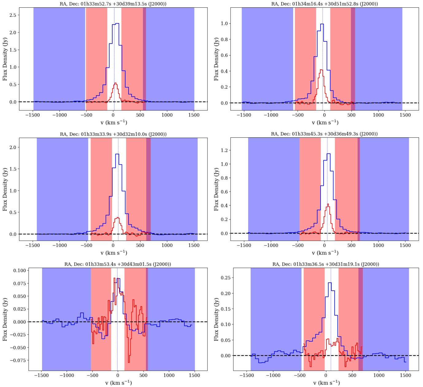
Fig. B.1. PACS spectra of [C II] (blue) and [O I](63 \mu\text{m} ) (red) at selected positions in M 33. All spectra are shown at their native angular resolution, before convolution to 12'' resolution. The velocities have been corrected for the systemic velocity of M 33 of -180 \text{ km s}^{-1} . Dashed, vertical lines mark the residual velocity of the H I line (Warner et al. 1973). Spectra are shown after subtraction of polynomial baselines of up to 3rd order. The two red (blue) fields mark the velocity range, which was used to calculate the baseline rms for the [O I] ([C II]) line. Baselines at more extreme velocities are not shown. [C II] integrated intensities were calculated over the inner range between the blue fields ( \pm 538 \text{ km s}^{-1} ), and the integrated intensities for the [O I] line were calculated over the spectral range (in white) between the red fields. The double-peak structure of the weak [O I] line seen in the right spectrum of the lower row is attributed to baseline noise.
