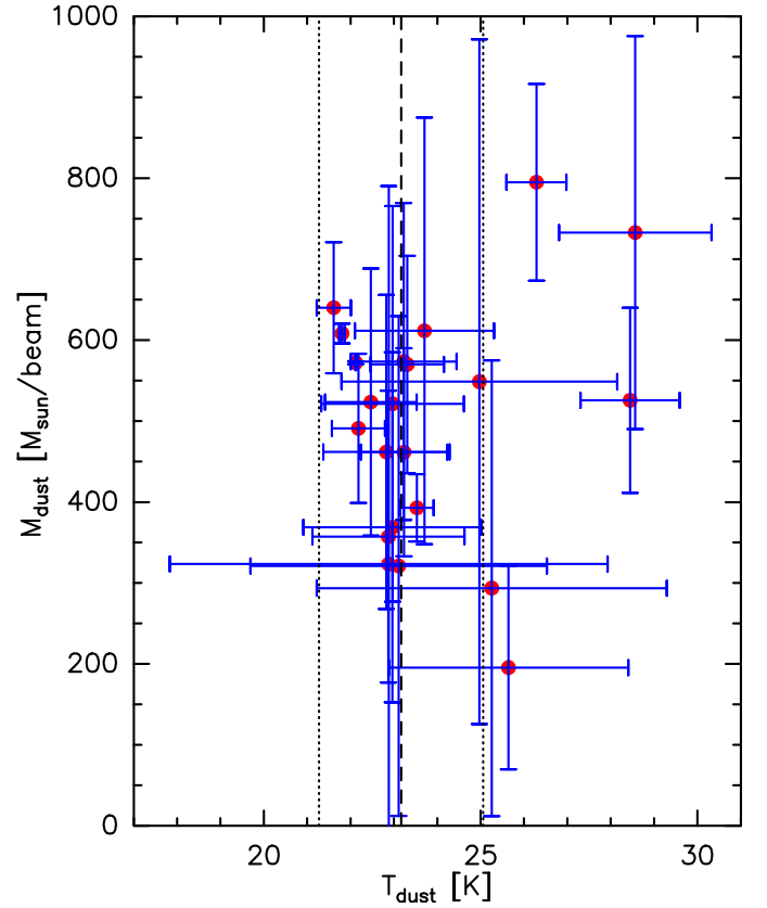
Fig. B.5. Dust mass surface density vs. dust temperature, derived from fits of modified black bodies, for the TIR bright positions in the H II region BCLMP 691. The thick dashed line shows the median dust temperature and thin dashed lines correspond to the rms scatter.
