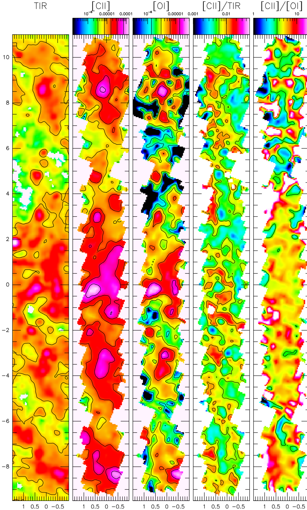
Fig. 2. Central part of the PACS maps of M33. From left to right: intensities of total infrared continuum (TIR), [C II], [O I](63 \mu\text{m} ), [C II]/TIR, and [C II]/[O I] intensity ratios. Intensities are in units of \text{erg s}^{-1} \text{cm}^{-2} \text{sr}^{-1} . Offsets are in arcminutes relative to the nucleus, after de-rotation of the position angle by 22.5^\circ . The TIR contour is at 2 \times 10^{-3} \text{erg s}^{-1} \text{cm}^{-2} \text{sr}^{-1} , the threshold intensity used in the correlation plots to distinguish TIR-bright and TIR-weak regions (Figs. 4–6, 8, 5). The color wedge is the same as in Fig. 1. [C II] contours are the same as in Fig. 1. [O I] contours are 1.4, 3.0, 6.3, 13.8 in units of 10^{-6} \text{erg s}^{-1} \text{cm}^{-2} \text{sr}^{-1} . The map of [C II]/TIR is overlaid with contours at the 0.6% and 1% level of the ratio. The map of [C II]/[O I] is overlaid with the contour of 3.5. Long tic marks in the color wedges indicate contour levels.
