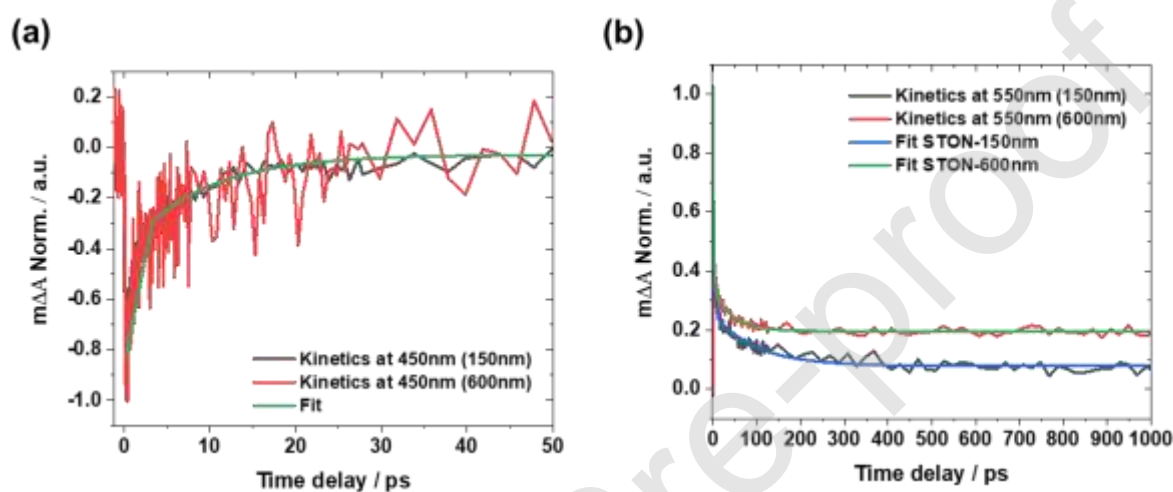
Figure 9. (a) Kinetics at 450 nm as a function of the delay and the thickness of STON films deposited on FG substrate and (b) kinetics at 550nm determined by femto pump-probe spectroscopy for an excitation at 330 nm.
