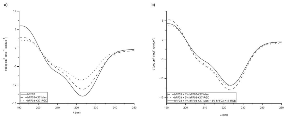
Figure 3. CD-spectra of 0.5 wt% peptide hydrogels directly after sample preparation at 37 °C. (a) pure peptide hydrogels, solid line – hFF03; dashes – hFF03-K17-Man; dotted – hFF03-K17-RGD (b) peptide hydrogel mixtures.
