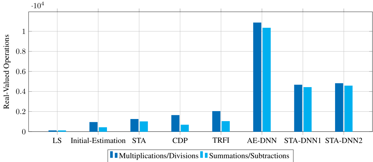
FIGURE 8: Computational complexity for different channel estimation schemes.
