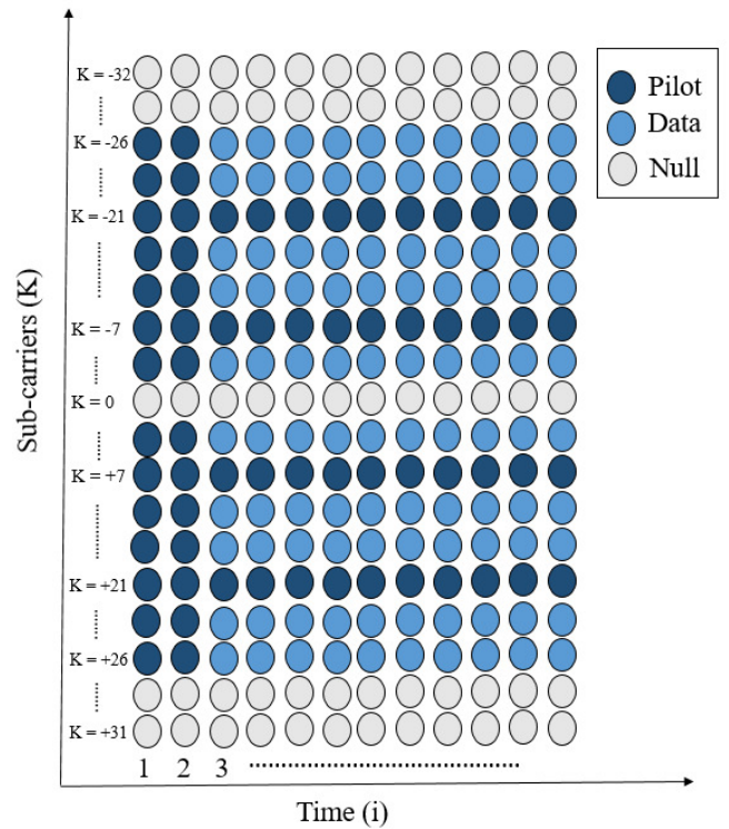
FIGURE 1: IEEE 802.11p subcarriers arrangement.
