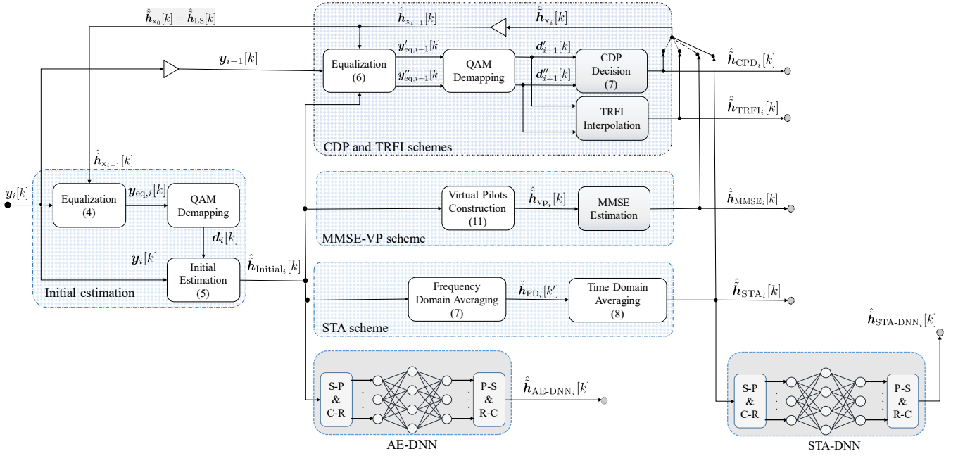
FIGURE 5: Proposed STA-DNN channel estimation scheme block diagram.
