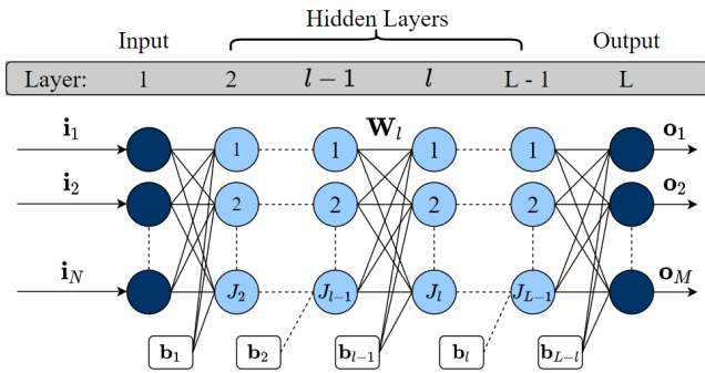
FIGURE 4: DNN architecture.
