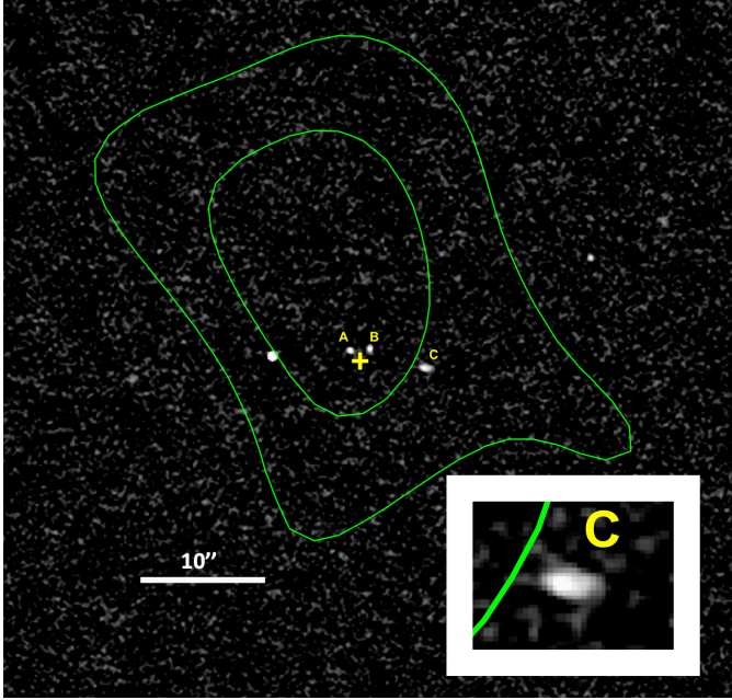
Fig. 8. X-ray contours (1 and 2\sigma ) from Chandra + XMM overlaid over the VLA 3 GHz image of the RO-1001 field. The offset between the X-ray peak and the Ly \alpha peak (yellow cross) is entirely consistent with arising from noise. The 3.1\sigma signal measurement is obtained integrating the emission over a region centered at the RO-1001 centroid and with 24'' radius (set to avoid a bright, unrelated point X-ray source that is increasing the noise substantially). The insert in the bottom-right corner shows a zoom onto source C, allowing a clear view of its elongated shape. The bright, left-most radio source is a low-redshift interloper.
