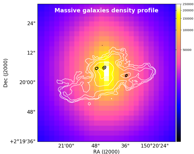
Fig. 9. Fourth-nearest neighbor projected density map of massive galaxies in RO-1001. Black contours are from ALMA detections. We note the excellent coincidence of the Ly \alpha emission (contours) with the potential well of the RO-1001 halo as traced by its massive galaxies. The color scale is in units of the number of galaxies per square degree.
