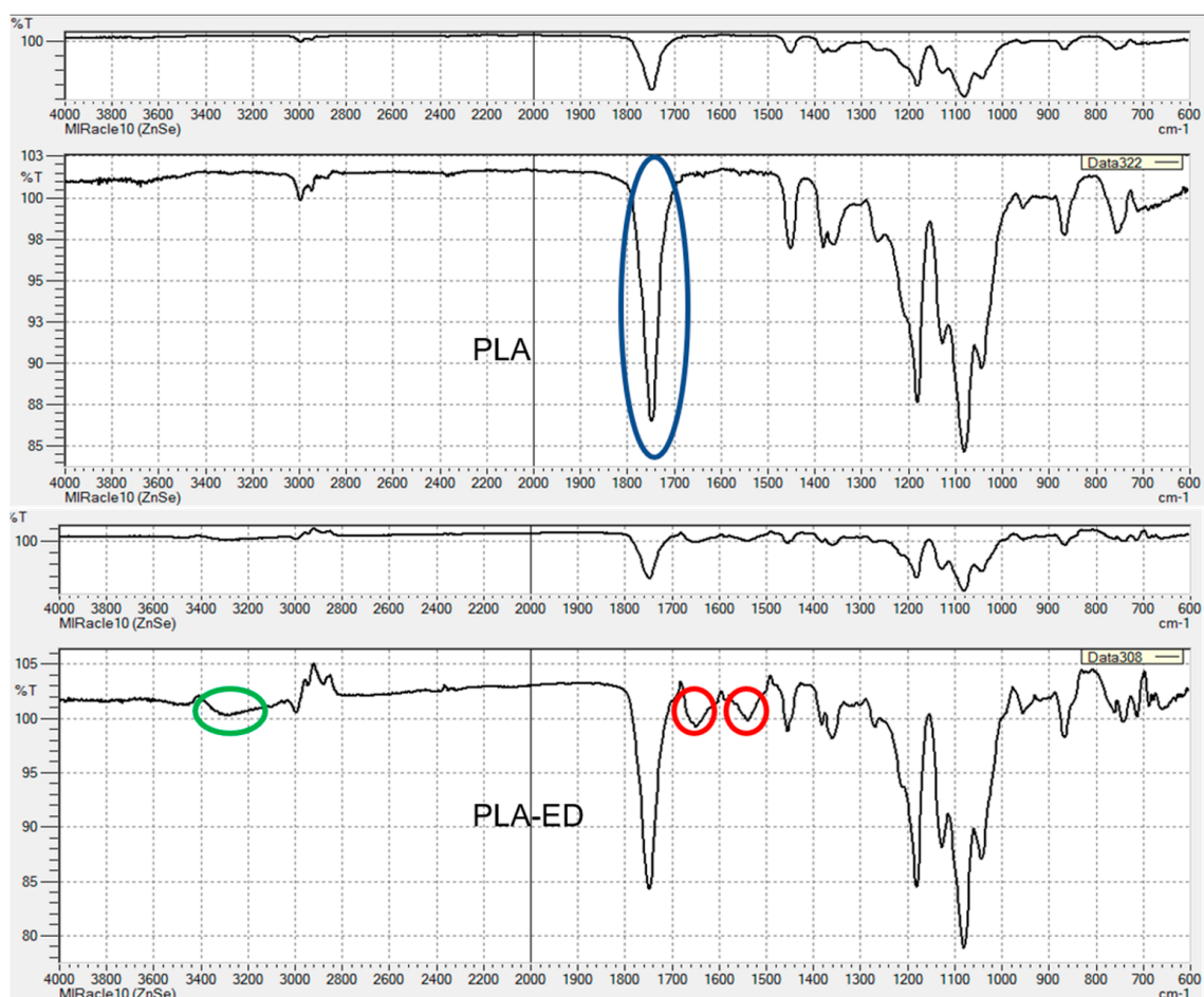
Figure 3. FT-IR spectra of PVTPs of PLA and PLA-ED. The ester C=O band is highlighted by a blue oval, the amide C=O bands by red circles, and the amide NH band by a green oval. From the presence of only the ester C=O stretch in PLA and the presence of both C=O amide and NH amide bands in the PLA-ED spectra, it is clear that the amide functionalization reaction has occurred, as was previously observed by time of flight secondary ion mass spectrometry (TOF-SIMS) for the surface modification of poly-ethylene-terephthalate (PET) by adenosine mono-phosphate (AMP) under the same conditions as in the current study [24].
