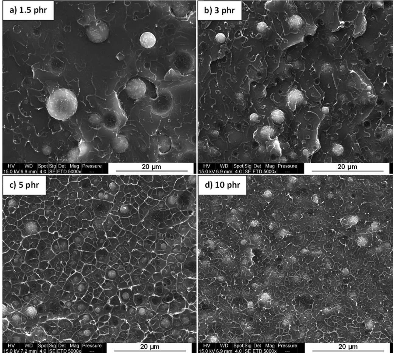
FIG. 2. SEM micrographs of PS/PA/JHNPs 80/20/X systems ( X = 1.5, 3, 5, and 10 phr) revealing particles agglomeration since 5 phr of JHNPs (the scale bar is 20 \mu\text{m} ).
