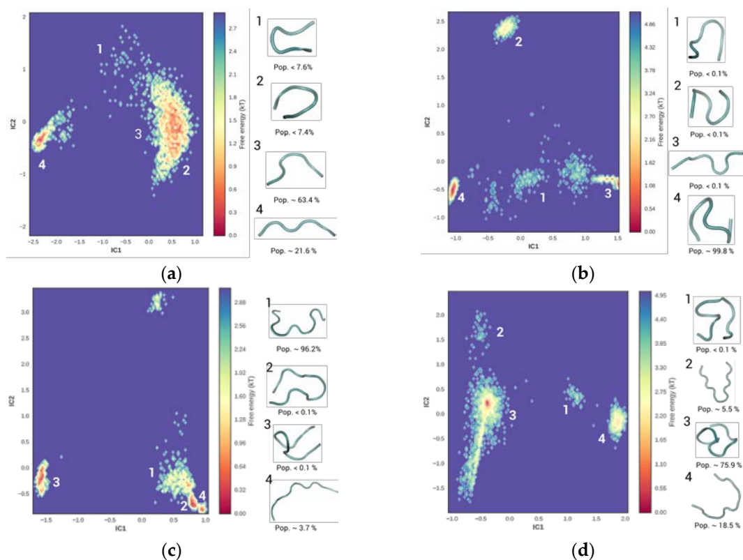
Figure 3. The free energy landscape and the four lowest energy configurations of the four peptides: (a) hexamer (SNLHPK); (b) octamer (CSIVEDGK); (c) NFO4 (VYMNRKYYKCCK); and (d) 13-mer (GPAGIDGPAGIRC) are illustrated. The equilibrium distribution of the folded peptide poses was provided as “Pop.” The scale bar indicates the basin depth of each contour feature, with bars towards the blue regime indicating the least favorable peptide configuration while the red regime indicates the most favorable peptide configuration. IC1 ( x -axis) and IC2 ( y -axis) represents the dimensional projection along the top two components of the IC analysis.
