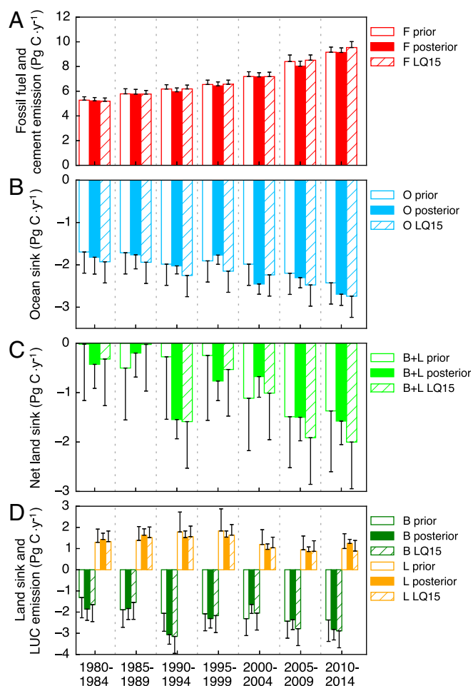
Fig. 2. (A) The fossil fuel and cement emissions (F), (B) ocean sink (O) and (C) net land flux (B + L), and (D) land sink (B) and land use change emissions (L) from prior knowledge, posterior results, and LQ15. All of the fluxes are 5-y means in each period. The error bars represent the 1- \sigma uncertainties.
