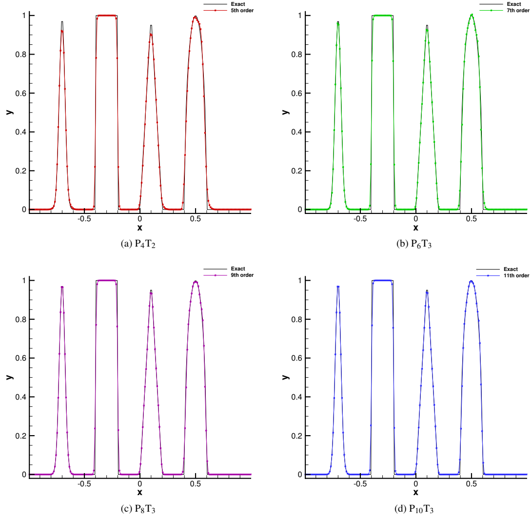
Figure 2: Numerical results for advection of complex waves. The numerical solutions at t = 2.0 with 200 mesh cells are presented.
