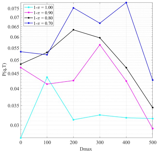
Fig. 2. Evolution of P(q, T) and R_{com} for different values of D_{max} and \pi , when \eta = 100 , the estimator (22) is considered for the dynamics of neighbors agents, as well as \mathbb{E} \left( \|e_i^j(t)\|^2 |k_j^{i,j} \right) from (58).
