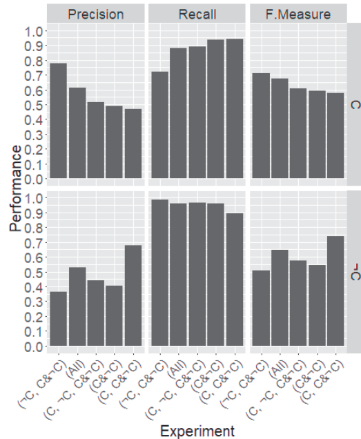
Fig. 1. Model performance for class C (top row) and \neg C (bottom row) when using different combinations of the patch category set, i.e. different distribution of the classes in the training set. Here, experiments are arranged according to the descending order of the precision on class C.
