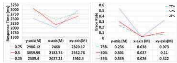
Figure 4: (Left): Study 1, Response time: Interaction between compression type and Compression Level . (Right): Study 1, Interaction effect on error rate; Between compression type and compression size.
