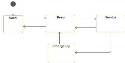
Figure 2: State values and transitions of the type of state operability
