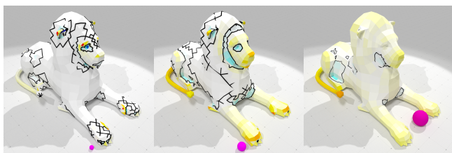
Figure 9: It is difficult to find a correct measuring ball radius \rho for normal cycle estimator \hat{H}^{nc} [CSM03], to be compared with \hat{H}^{cnc} result on Figure 10.
