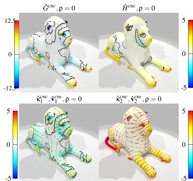
Figure 10: Gaussian, mean and principal curvatures and directions with our method on Lion dataset.
