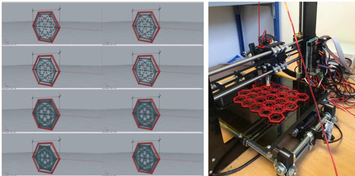
Figure 6. Left: Simulation and Physical Properties: A Single component's performance simulations to study Alkaline Hydrolyzed Polyacrylonitrile (HPAN) behavior with Ni-ti alloy as actuator components going from tension to relaxation. Simulation executed using Rhinoceros 5.0 + Grasshopper version (0.9.0076) + Kangaroo (version 0.099). Right: Test 3D-printing prototype of a 5 X 5 cell - patches 25 .
