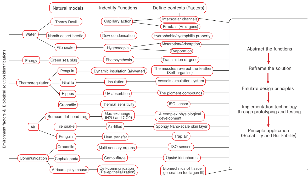
Figure 4. The unique flow chart methodology leading to a concept design of the living envelope.
