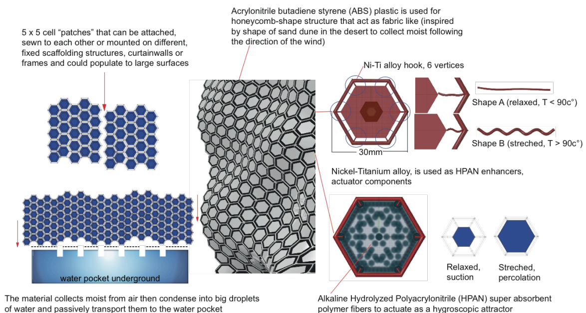
Figure 5. Hygro-NET system diagram, fog-harvesting material that behaves as functional living system.
