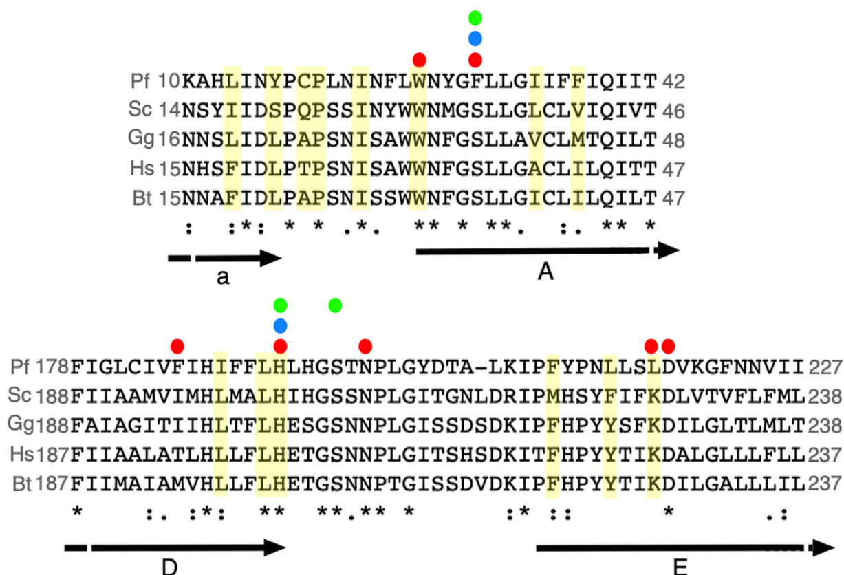
Fig. 5. Protein sequence alignment of the Q_i -site region of cytochrome b from Plasmodium falciparum (Pf, UniProtKB accession: Q02768), Saccharomyces cerevisiae (Sc, P00163), Gallus gallus (chicken, Gg, P18946), Homo sapiens (Hs, P00156) and Bos taurus (cow, Bt, PB00157). Sequence conservation in the aligned sequences is indicated using the CLUSTAL OMEGA convention [144], with asterisks, colons and periods indicating complete conservation, conservative substitutions and semi-conservative substitutions, respectively. Sequence data were obtained from the UniProt database. Arrows underneath the alignment indicate \alpha -helices as identified in Fig. 3. Residues in the bovine cytochrome b atomic structures 1NTK [35], 4D6T [5] and 4D6U ( ibid ) in potential hydrogen-bonding association with bound antimycin, and the 4(1H)-pyridones GW844520 and GSK932121 are indicated by red, blue and green circles, respectively. Residues forming stabilising hydrophobic contacts with bound GW844520 in the bovine 4D6T structure are shaded in yellow. (GSK932121 displays similar binding interactions.) Protein–ligand associations indicated in this figure were predicted and analysed using the LPC software package [145].
