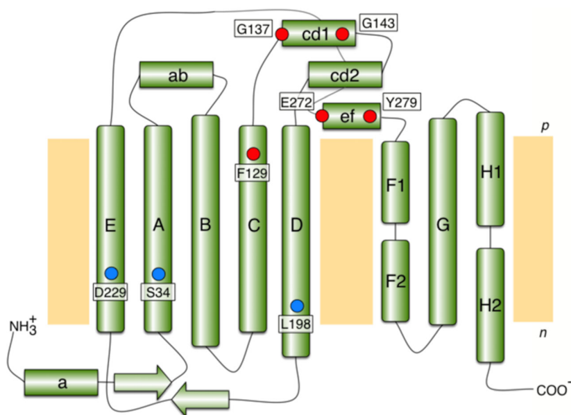
Fig. 3. Cartoon of the secondary structure and membrane disposition of cyt b , displaying the location of Q_o (red) and Q_i (blue) residues of interest ( Saccharomyces cerevisiae notation) as discussed in the text. Transmembrane and surface helices are identified in upper and lower cases, respectively. 'n' and 'p' refer to the negative and positive sides of the energised inner mitochondrial membrane.
