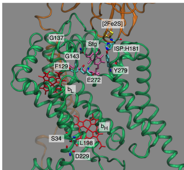
Fig. 1. Cartoon representation of the atomic structure of cyt b (green) and the ISP (orange) of yeast cyt bc 1 (1EZV.PDB [39]) with stigmatellin (Stg, pink) bound at Q o . The ISP [2Fe2S] cluster, cyt b haems (red) and side chains of interest as discussed in the text are represented in wireframe form.
